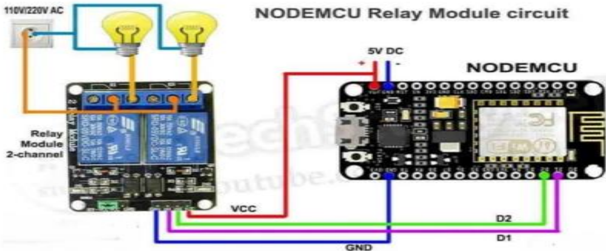
Fig : Circuit Diagram
