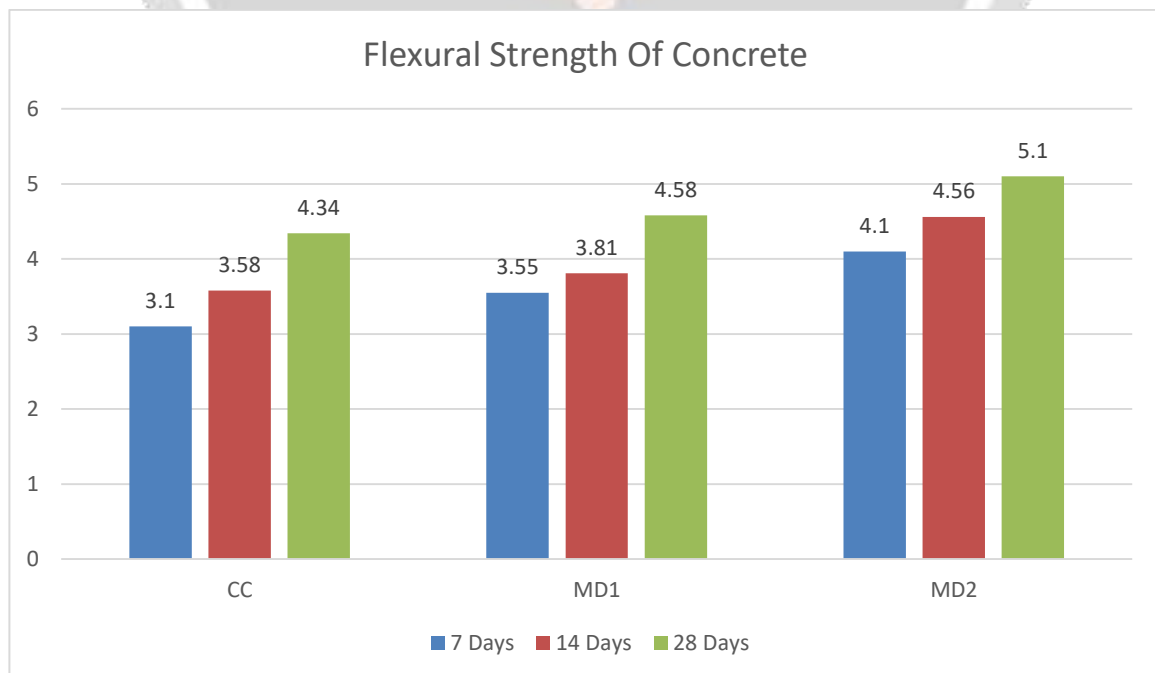
Fig 2- Flexural Strength Test
