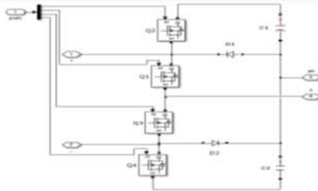
Fig-12: conventional dc-dc converter
