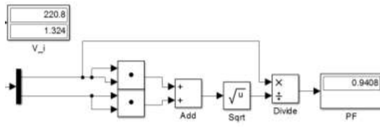
Fig-19: Power factor of the conventional system
