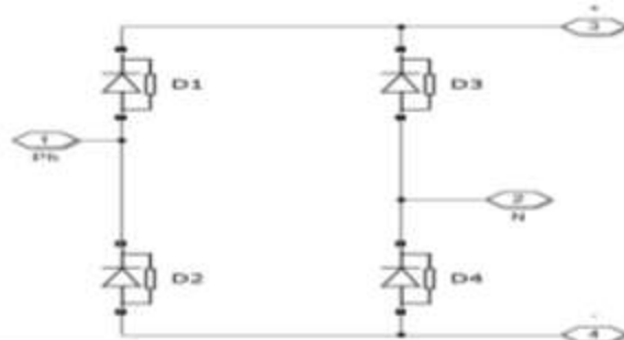
Fig-11: diode rectifier drawn using matlab design
