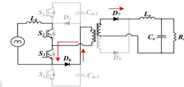
Fig-7: Operation mode of the converter Mode 8: t8 < t < t9 .
