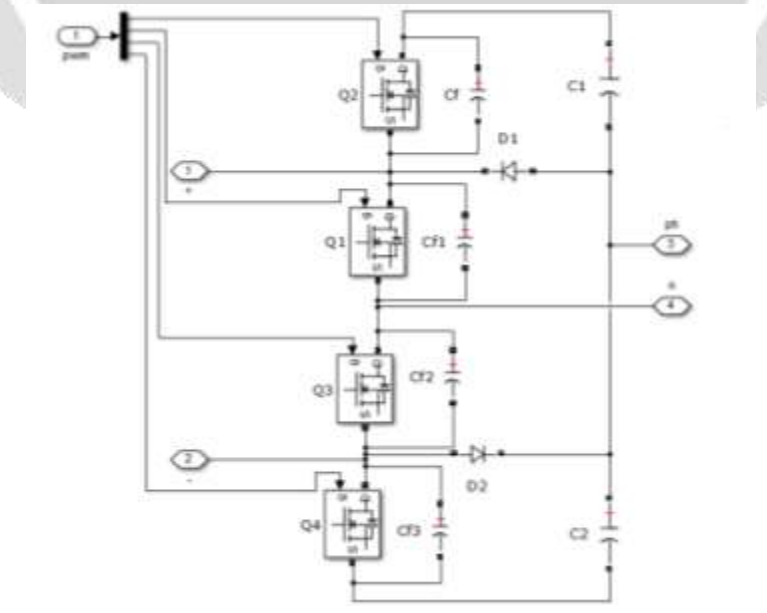
Fig-3: Proposed DC-DC converter with capacitors across each switch.
