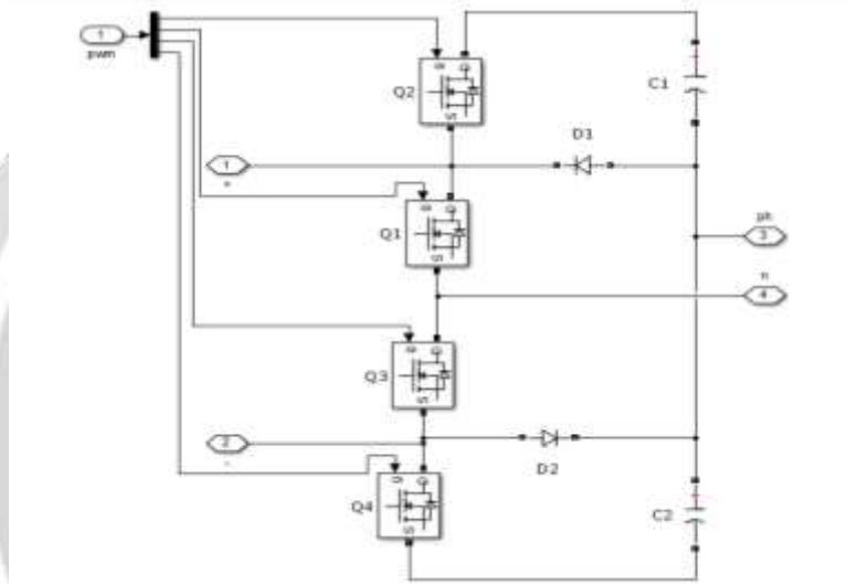
Fig-2: Conventional DC-DC converter
