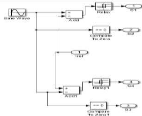
Fig.22 PWM generation using hysteresis loop
