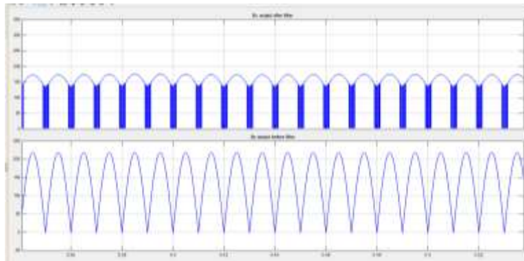
Fig-15: rectified sine waveform before filter inductor
