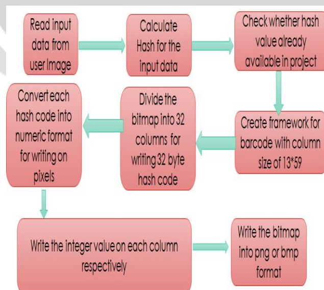
Fig.3 Barcode Generation
