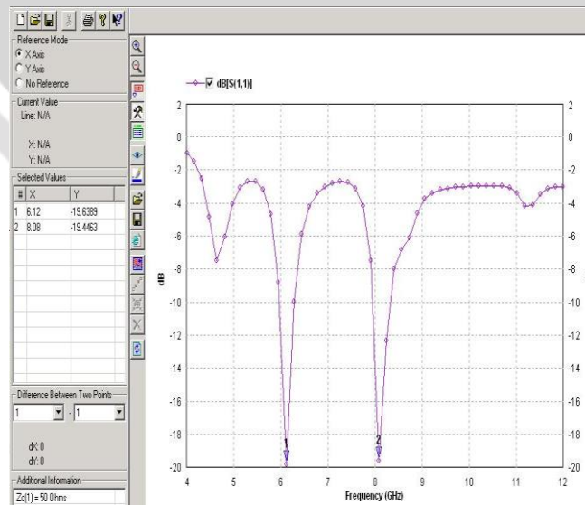
Fig - 9: Return Loss of Second Order
