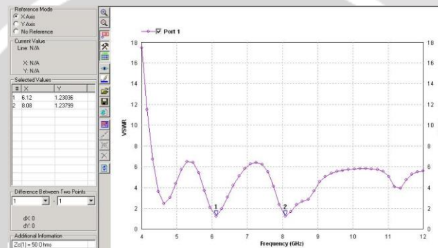
Fig – 6: VSWR of Base Shape
