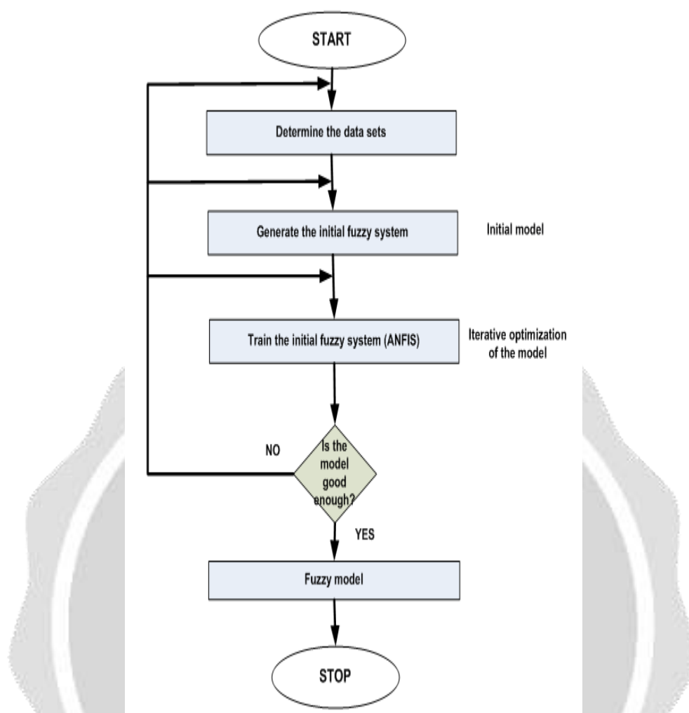
Figure 3: fuzzy modeling.
