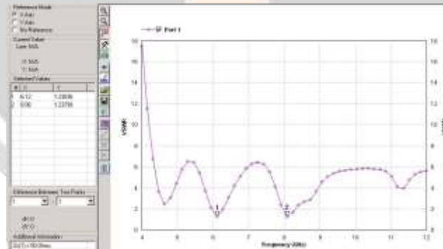
Fig. 7. VSWR of First Order
