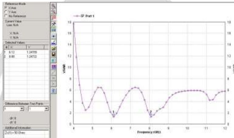
Fig. 10. VSWR of Second Order
