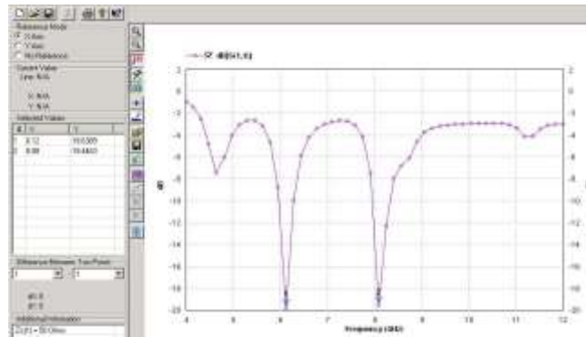
Fig. 9. Return Loss of Second Order
