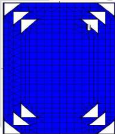
Fig. 4. Third Order Shape of triangularly slotted fractal Antenna
