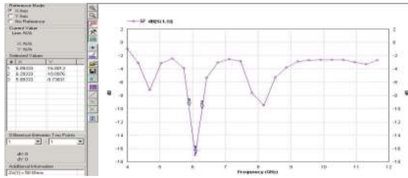
Fig. 5. Return Loss for Base Shape
