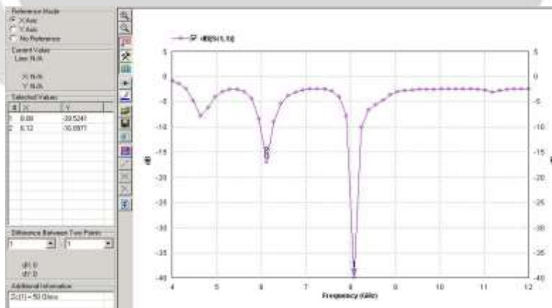
Fig. 11. Return Loss for Third Order
