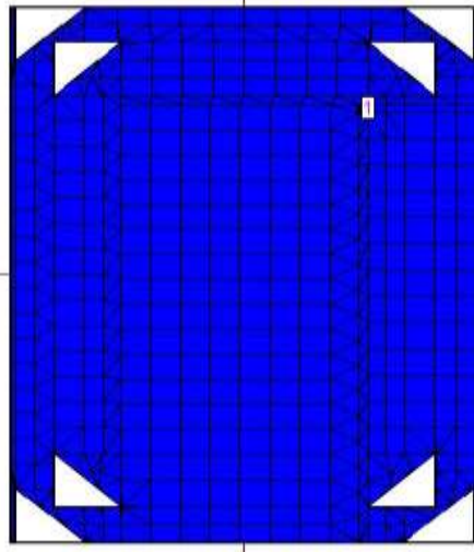
Fig. 3. Second Order Shape of triangularly slotted fractal Antenna
