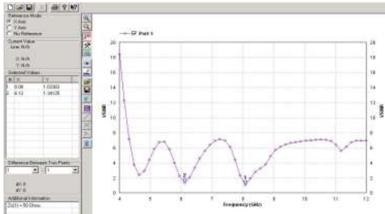
Fig. 12. VSWR of third order
