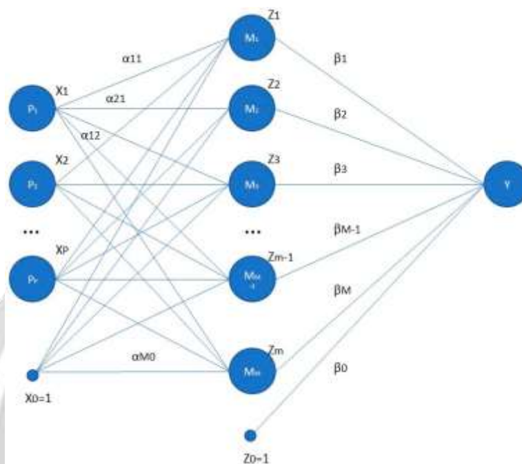
Figure 1. ANN structure.
