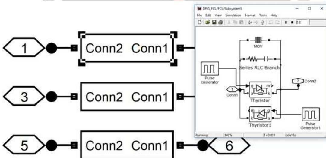
Figure 3.2 Proposed FCL Subsystems.
