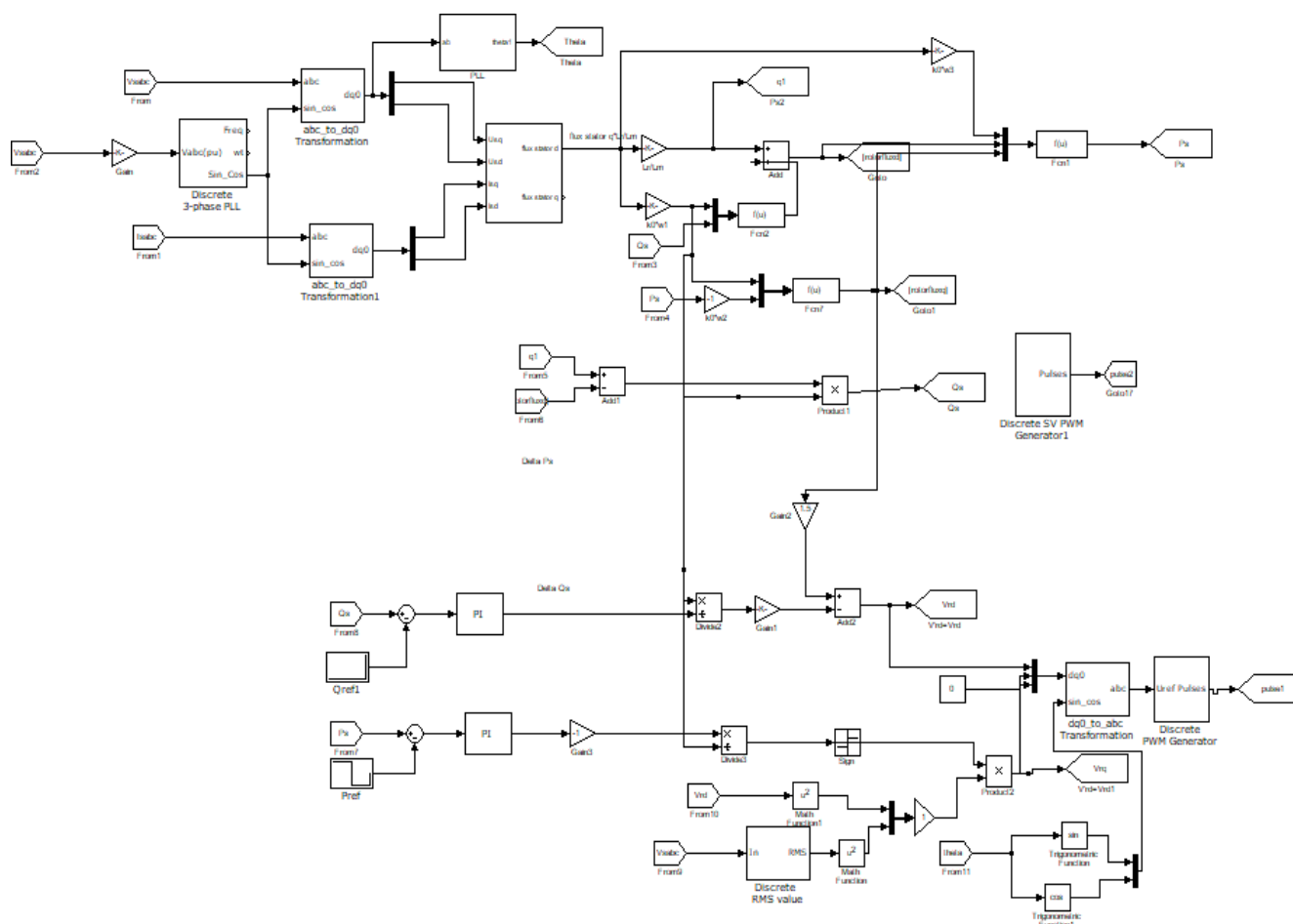
Figure 3.3 Proposed Control Loop.
