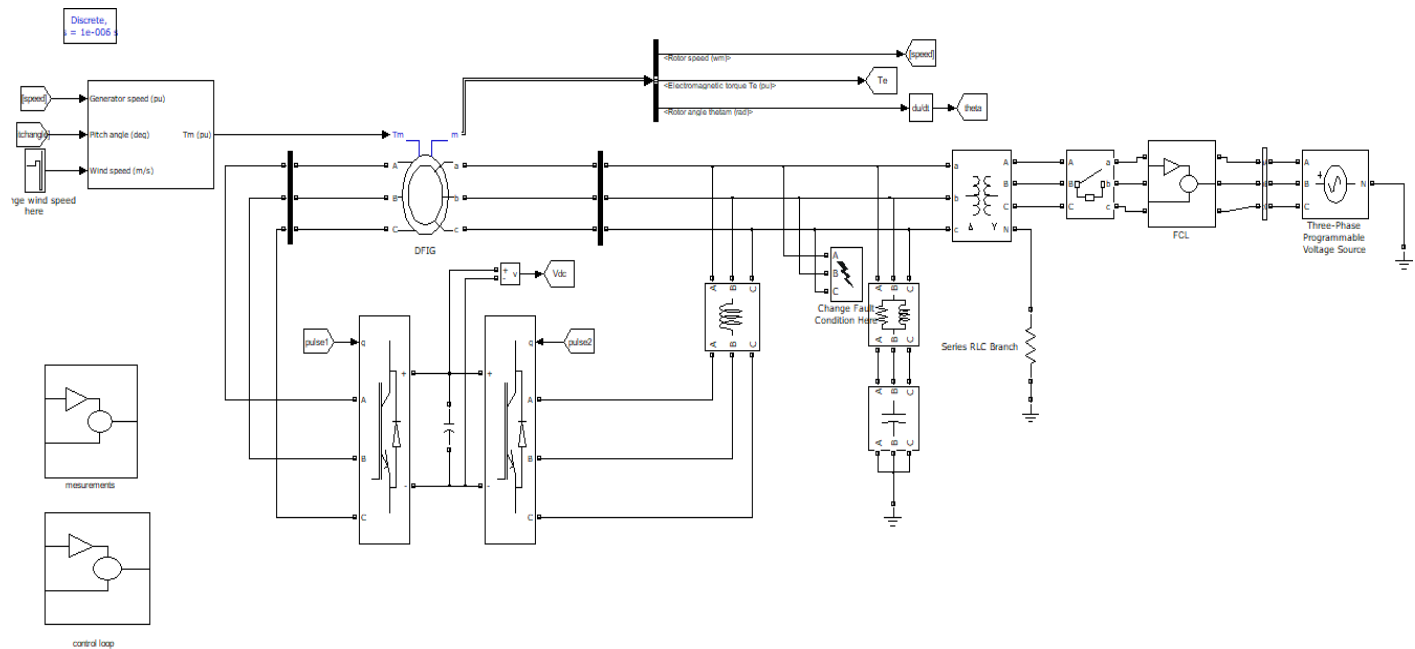
Fig. 3.1 Proposed System Design with FCL extension.
