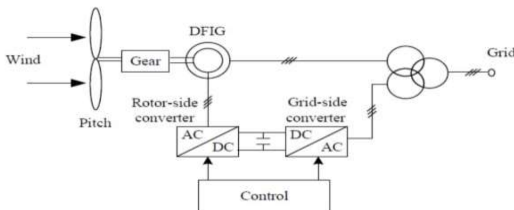
Figure 2.1 DFIG wind turbine configuration.
