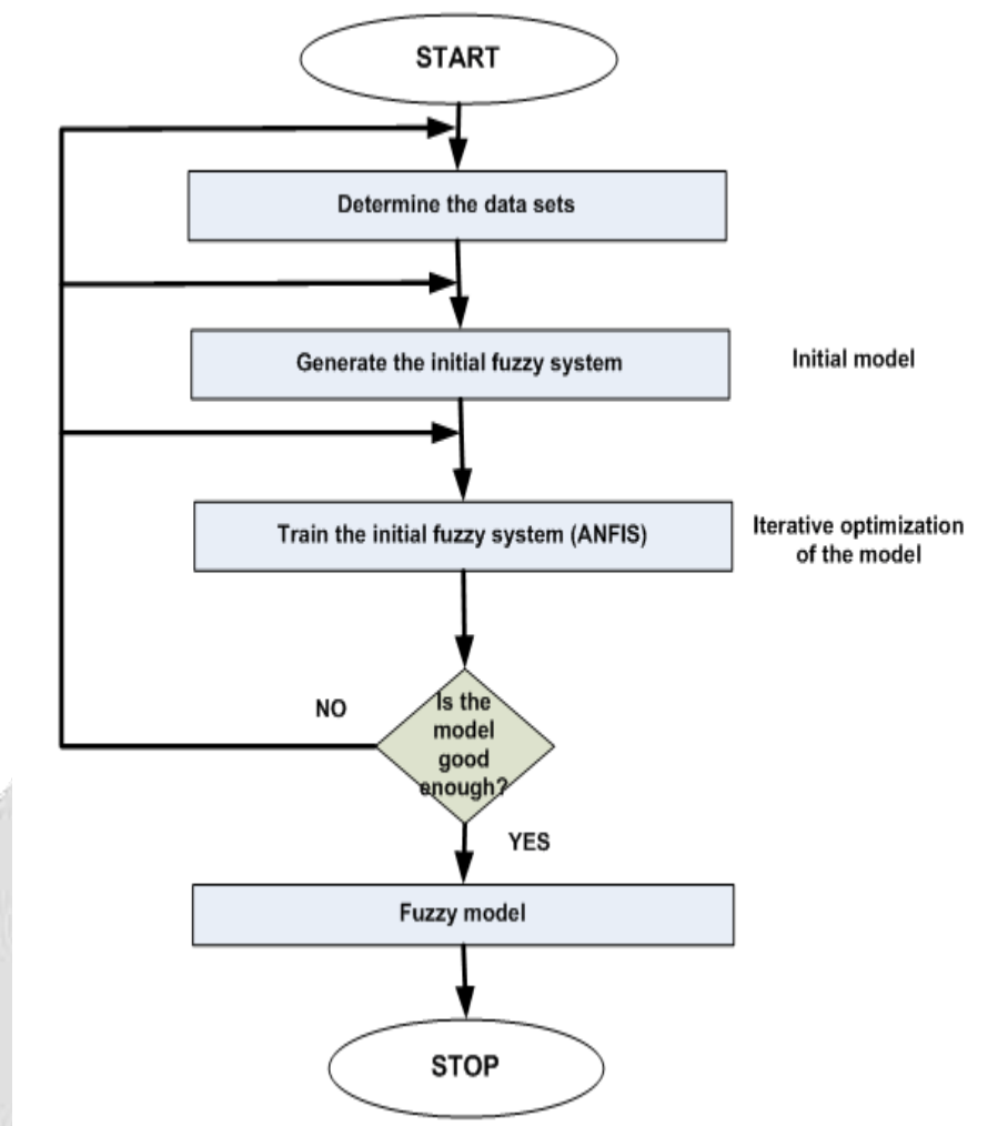
Figure 2: fuzzy modeling.
