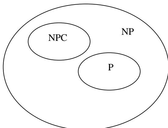
Fig. 2 : NP hard and complete NP-complete
