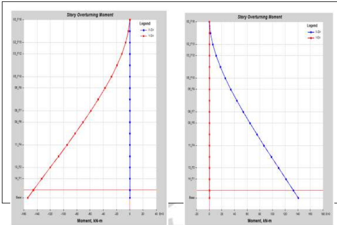
Fig.6.2(e) Story Moments at X and Y direction Due to load EQx and EQy
