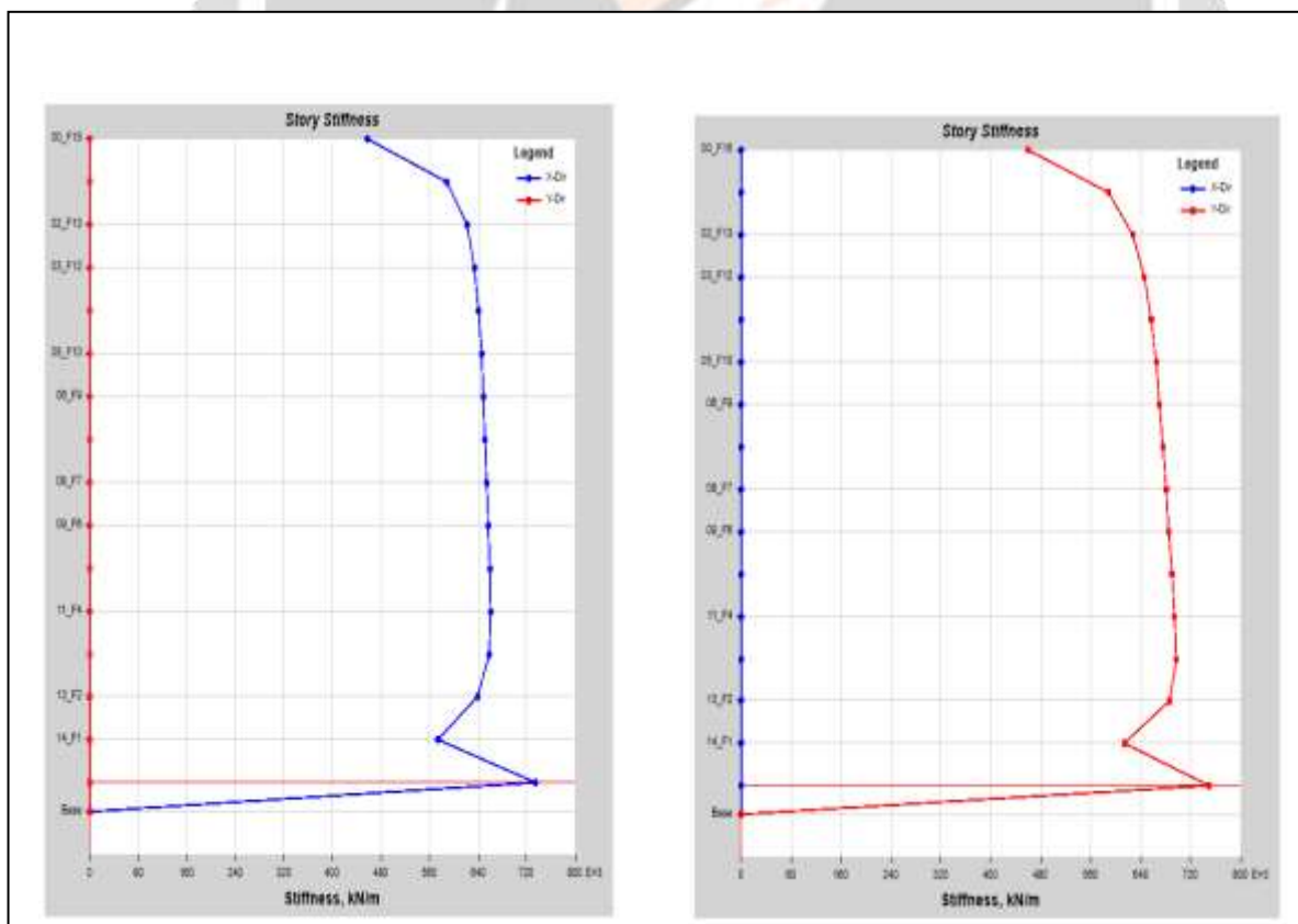
Fig.6.1(d) Story Stiffness at X and Y direction Due to load EQx and EQy
