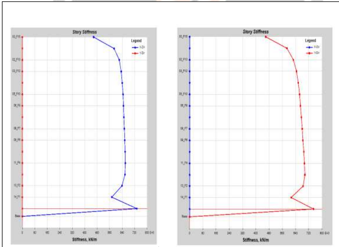
Fig.6.2(d) Story Stiffness at X and Y direction Due to load EQx and EQy
