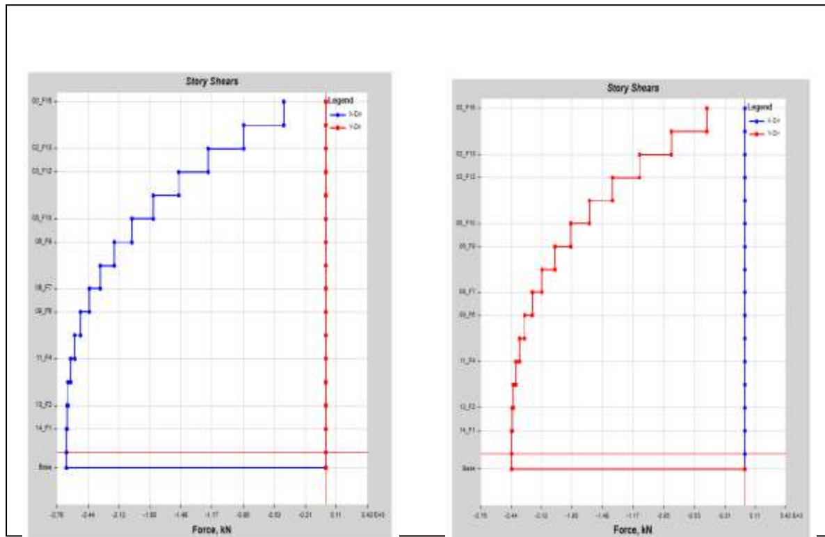
Fig.6.1(c) Story Shear at X and Y direction Due to load EQx and EQy
