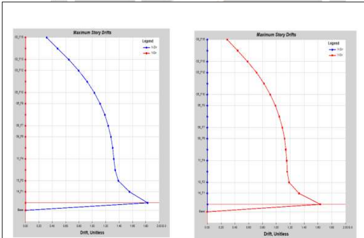
Fig.6.1(f) Story Drifts at X and Y direction Due to load EQx and EQy
