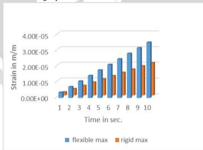
Graph 3 – Strain in flexible and rigid pavement.
