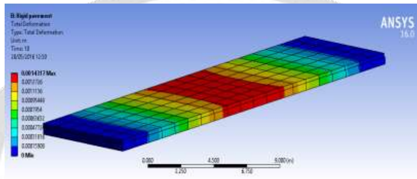
Fig. 6 Total deformation of rigid pavement.
