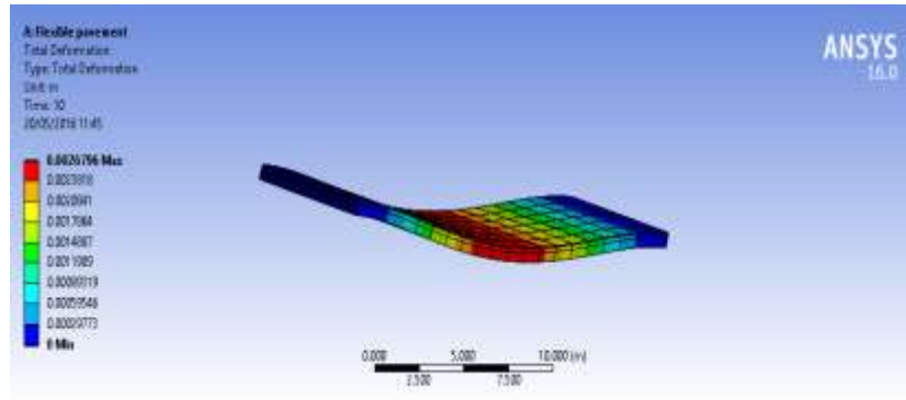
Fig. 5 Total deformation of flexible pavement.
