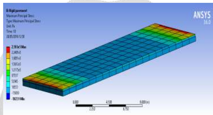
Fig. 8 Stresses in rigid pavement.
