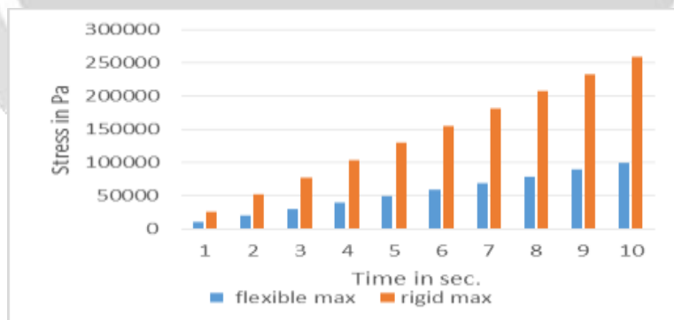
Graph 2 – Stresses in flexible and rigid pavement.
