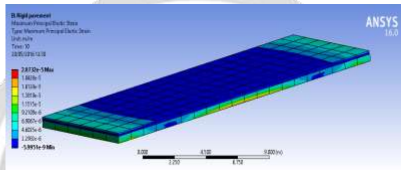
Fig. 10 Strain in rigid pavement.
