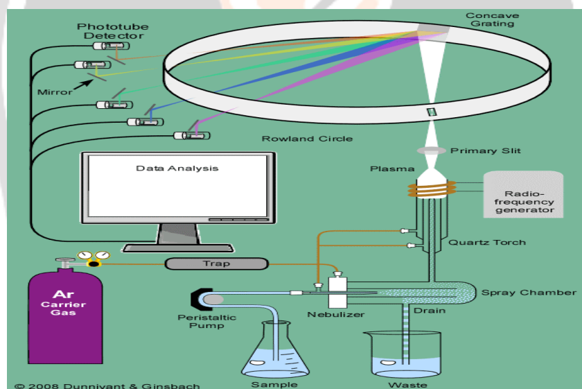
Fig- 4: Inductively coupled plasma-atomic emission spectrometry (ICP-AES)
