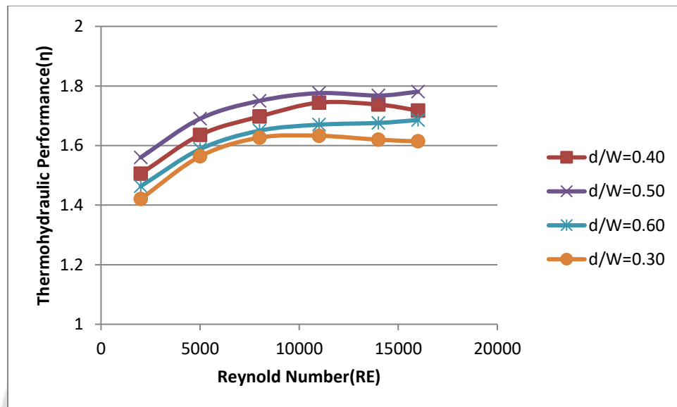
Figure No. 7 Thermo-hydraulic performance parameter as a function of Reynolds Number for different relative gap position ( d/W )
