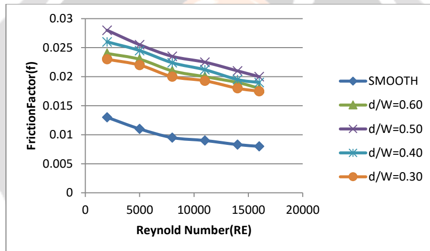
Fig. 6 Variation of Friction factor and Reynolds number at different gap position ( d/W )
