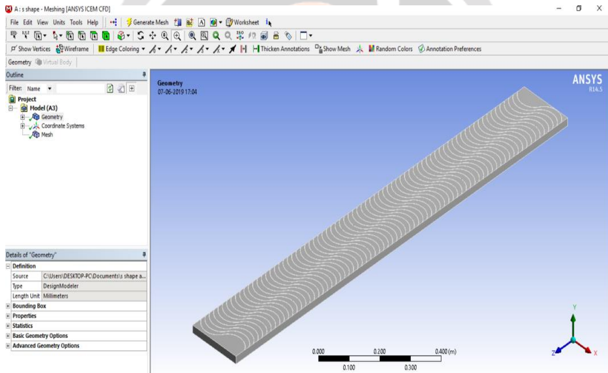
Fig. 2 Geometry of Broken 'S' arc rib
