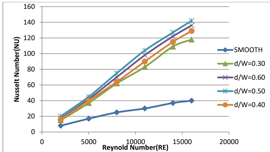
Fig. 4. Variation of Nusselt number with Reynolds number for different Values of relative gap position ( d/W ).
