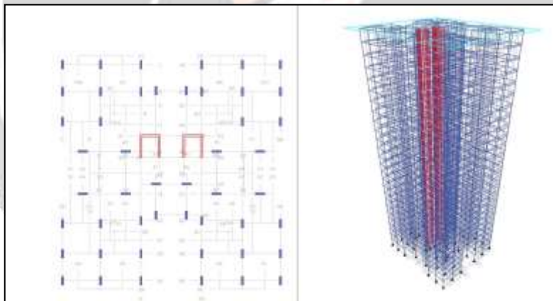
Fig -1: Plan and Elevation of G+25 RC multistoried framed Building in ETABS2013
