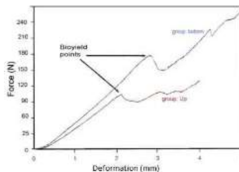
Figure 2. Typical force-deformation curve for strength in compression experiment.
