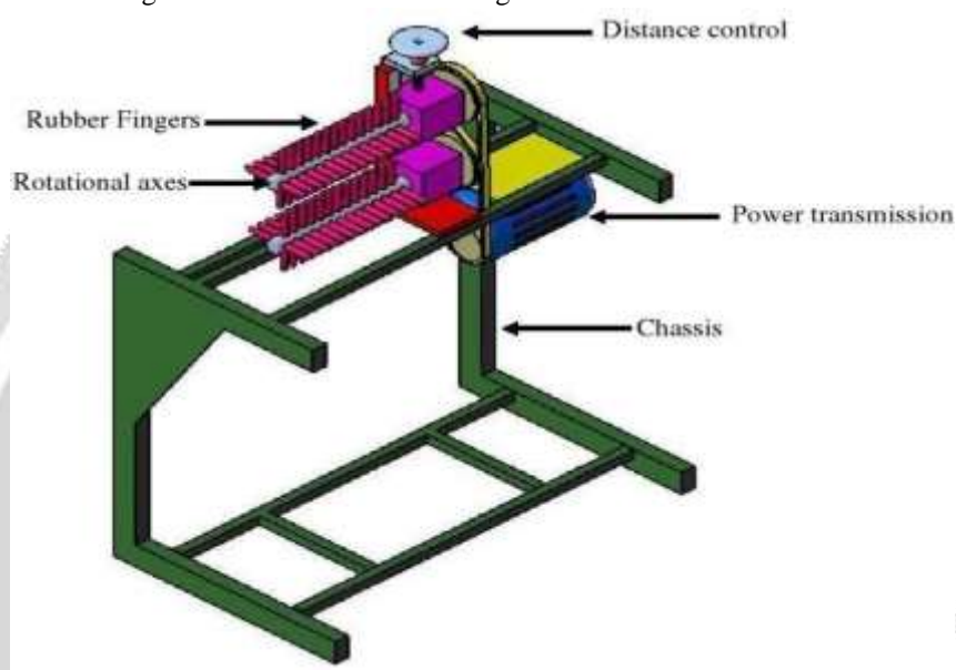
Figure1. Schematic of Leaf cutter machine
