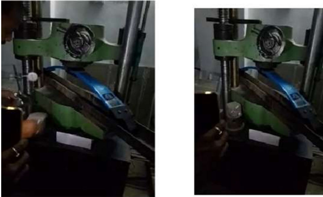
Fig.8.1 Testing of Composite Leaf spring on UTM
