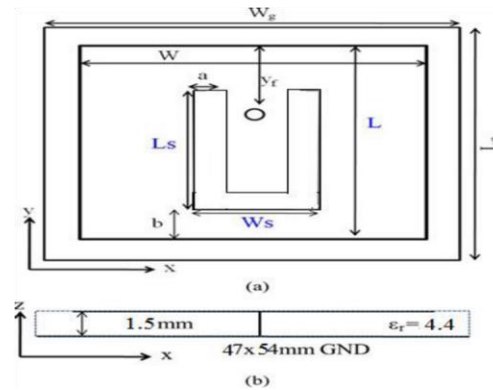
Figure 3: The geometry of quad-band U-slot microstrip patch antenna [7]
