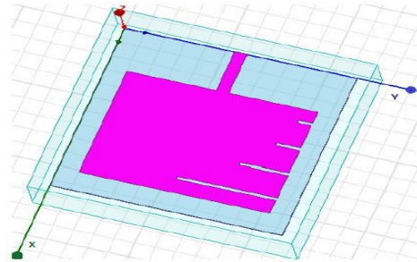
Figure 5: low-profile compact microstrip patch antenna [9]
