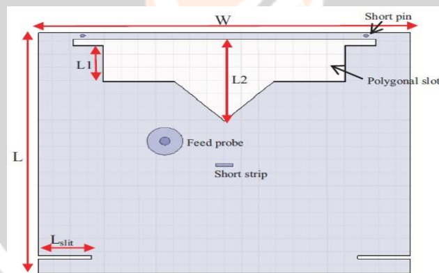
Figure 2: Configuration view of tri-band antenna[6]
