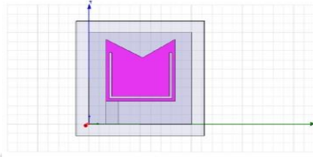
Figure 1: M-shape microstrip antenna [5]
