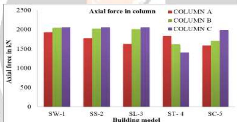
Fig. 17 Axial forces in column for building on sloping ground
