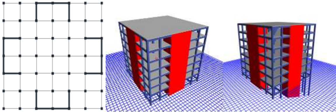
Fig. 7 Building with Channel-shape shear walls on plain and sloping ground
