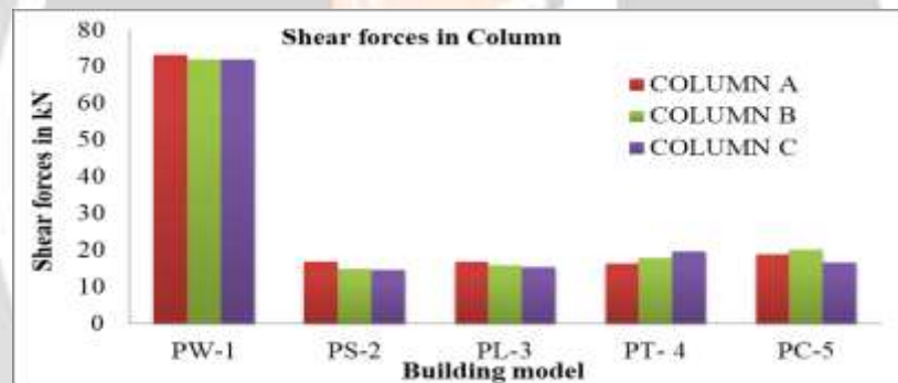
Fig. 12 Shear forces in column for building on leveled ground
