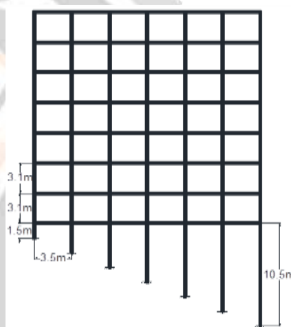
Fig. 2 Building frame on sloping ground
