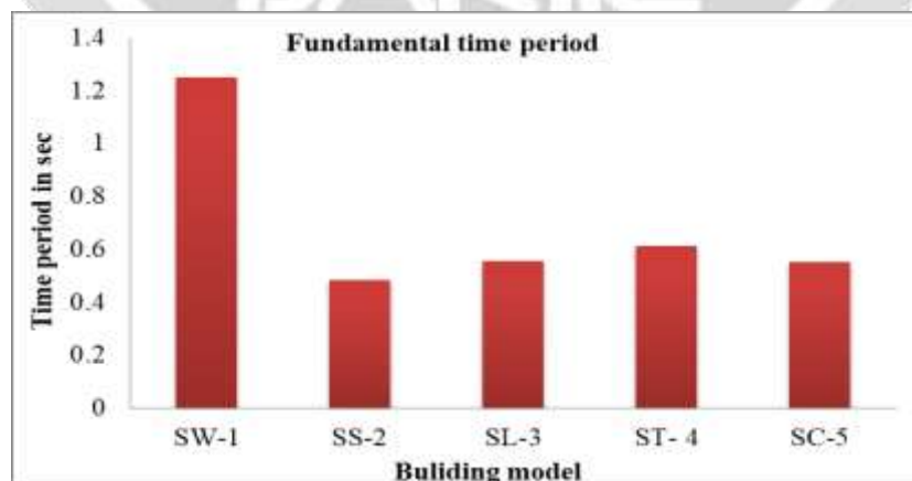
Fig. 15 Variation of time period for building on sloping ground
