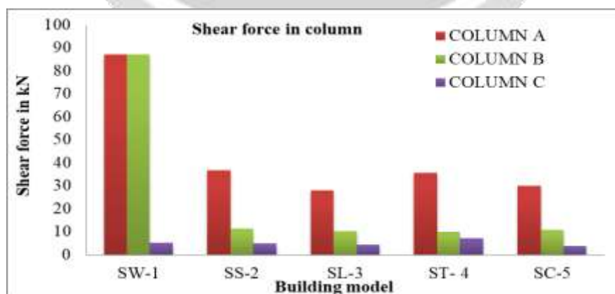
Fig. 18 Shear forces in column for building on sloping ground
