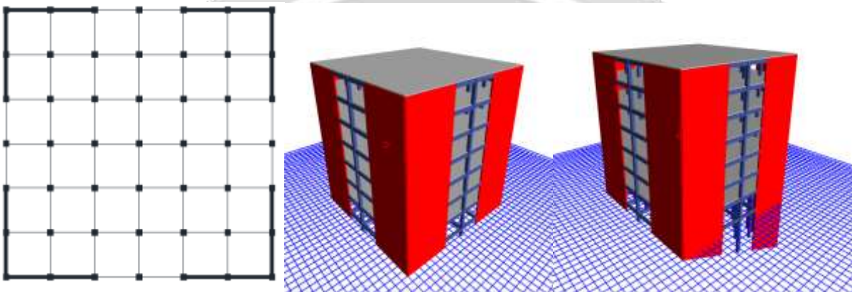
Fig. 5 Building with L-shape shear walls on plain and sloping ground
