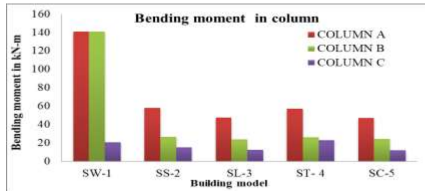
Fig. 19 Bending moment in column for building on sloping ground
