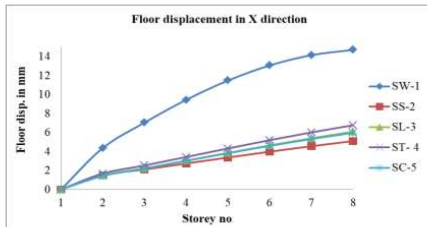
Fig. 16 Lateral displacement of building on sloping ground
