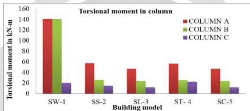
Fig.20 Torsional moment in column for building on sloping ground
