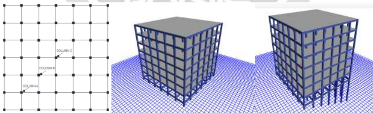
Fig. 3 Building without shear wall on plain and sloping ground
