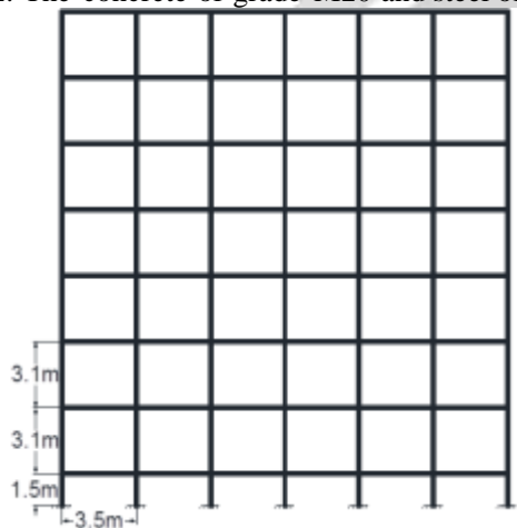
Fig. 1 Building frame on leveled ground
