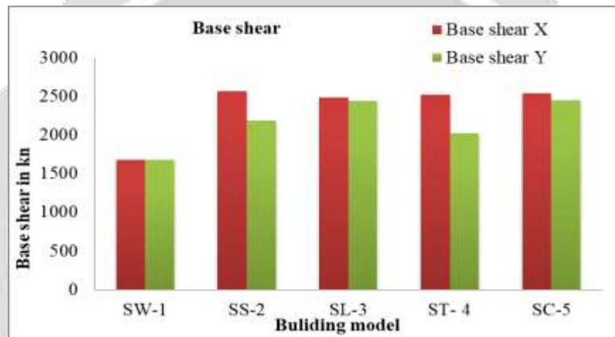
Fig. 14 Variation of base shear for building on sloping ground
