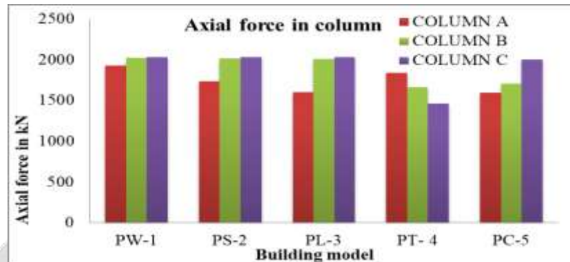
Fig. 11 Axial forces in column for building on leveled Ground
