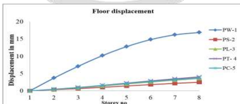
Fig.10 Lateral displacement of building on leveled ground.
