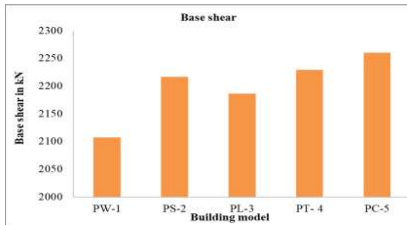
Fig. 8 Variation of base shear for building on leveled ground
