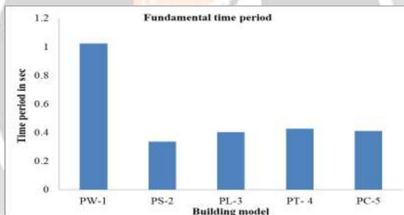
Fig. 9 Variation of time period for building on leveled ground
