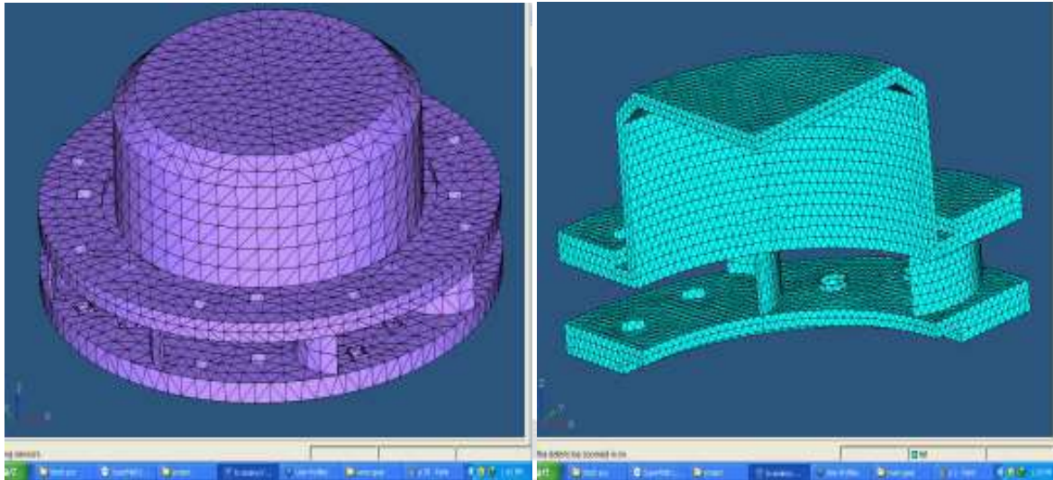
Fig.4 Meshing
