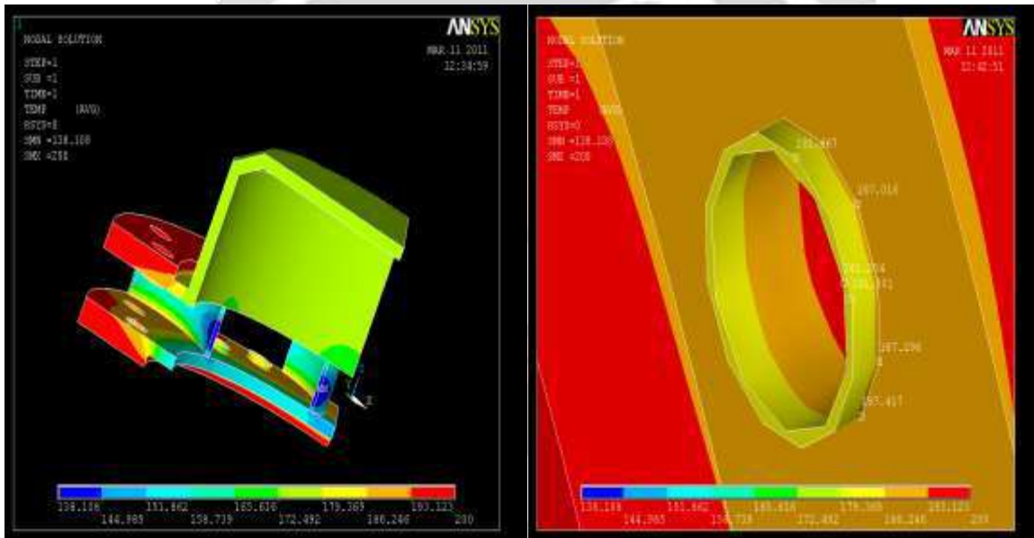
THERMAL ANALYSIS OF CAST IRON
