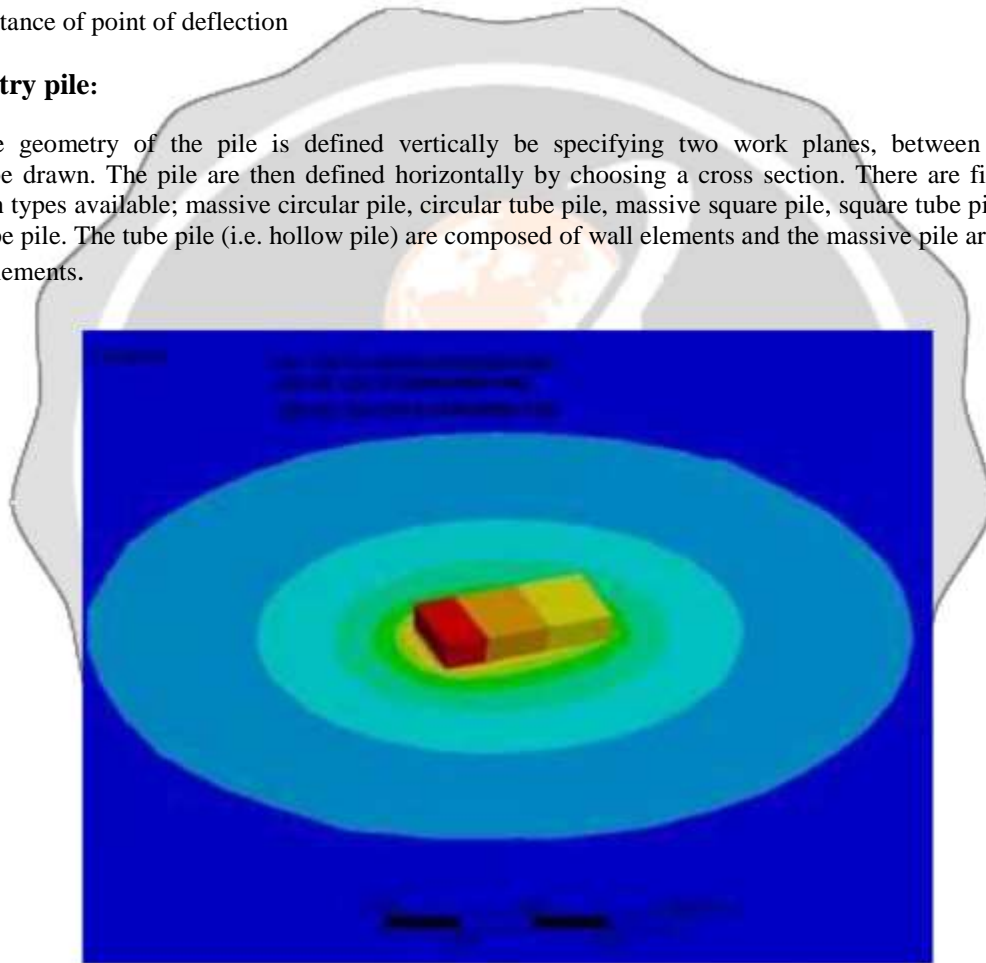
ANSYS Typical plan of soil profile & pile group foundation modeling.
