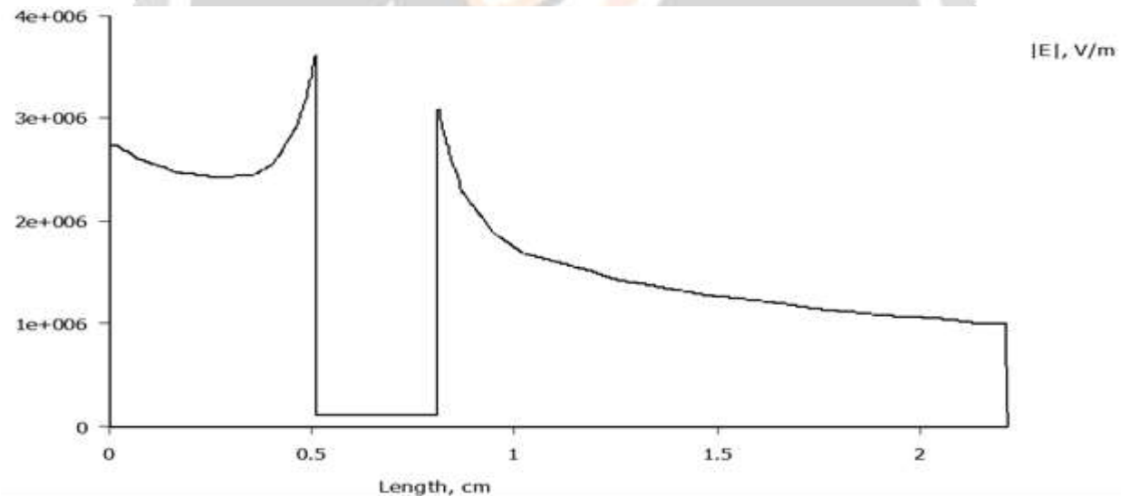
Fig 6: Electric field distribution with water cavity (permittivity=78.5)
