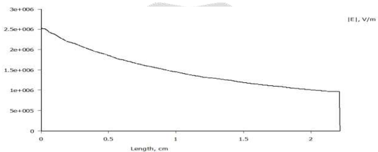
Fig 2: Electric Field Distribution without Cavity
