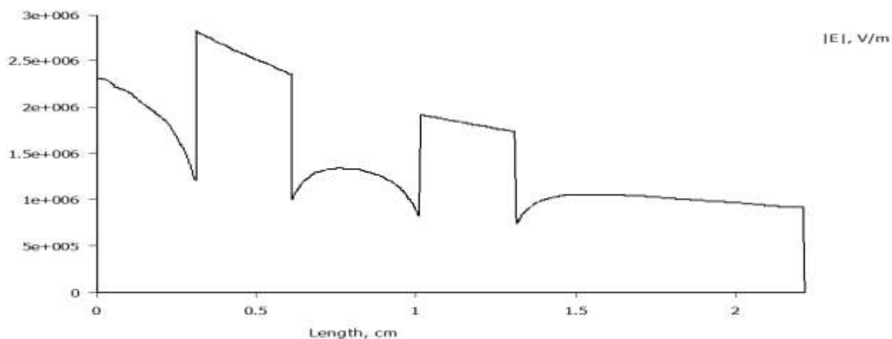
Fig 4: Field Distribution in presence of cavity at different locations (Axially)
