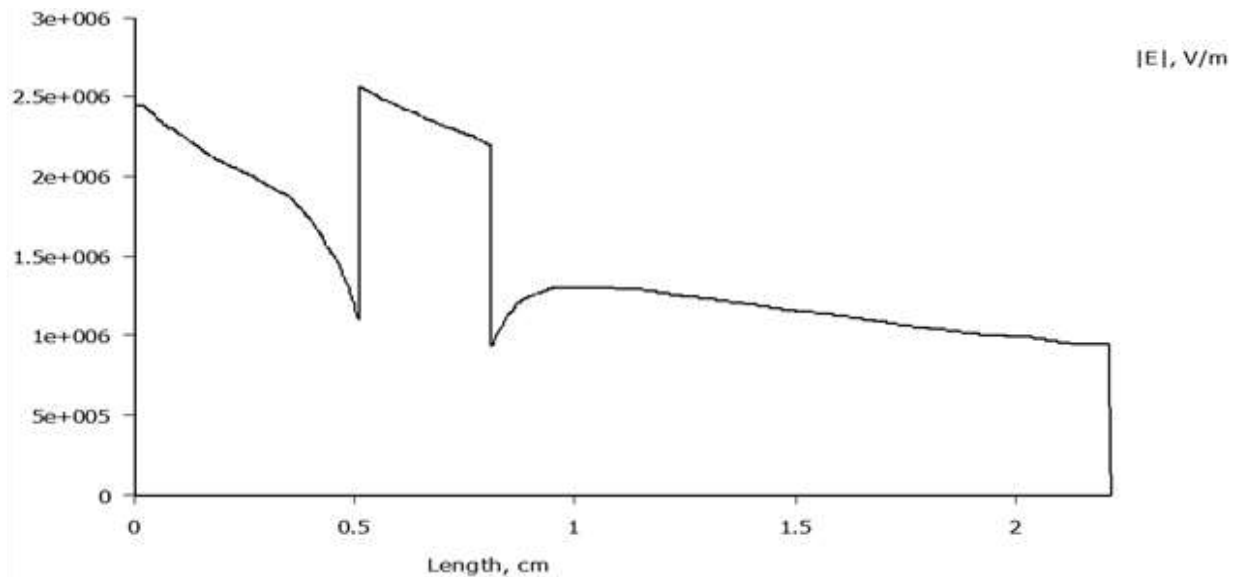
Fig 5: Electric field distribution with water cavity (permittivity=1)
