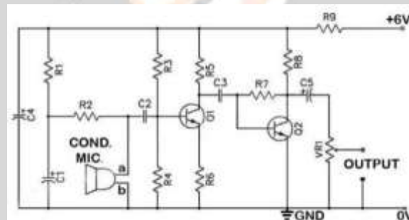
Fig.7 Sound sensor
