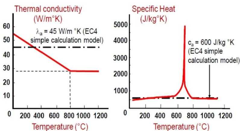
Fig. 1. Thermal properties of steel
