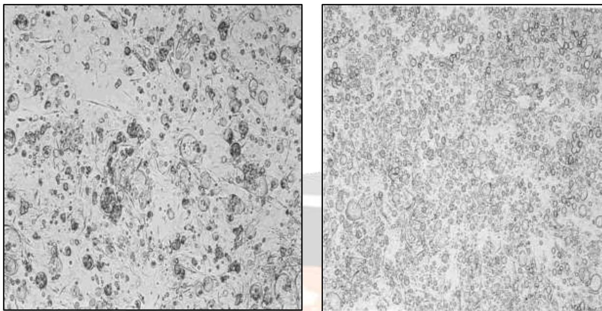
Fig 1: a) Image of MLV liposomes of Acitrecin and Methotrexate b) Image of SUV liposomes of Acitrecin and Methotrexate (200 X).
