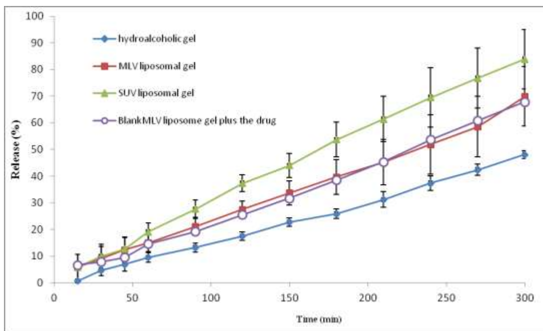
Fig 2: The percentage release of Acitrecin and Methotrexate from different gel formulations
