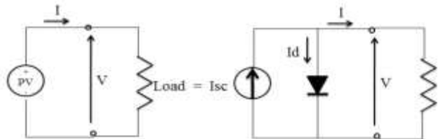
Fig-1: Equivalent circuit of photovoltaic cell
