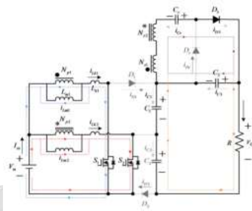
Fig-4: First stage
