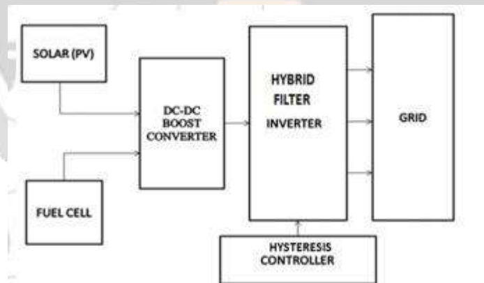
Figure 9: Block diagram of hybrid system
