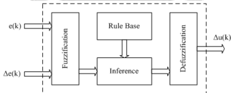
Figure 2: Structure of Fuzzy logic controller
