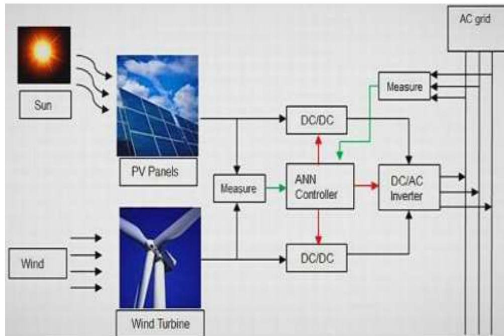
Figure 6 : Hybrid power system with neural network controller
