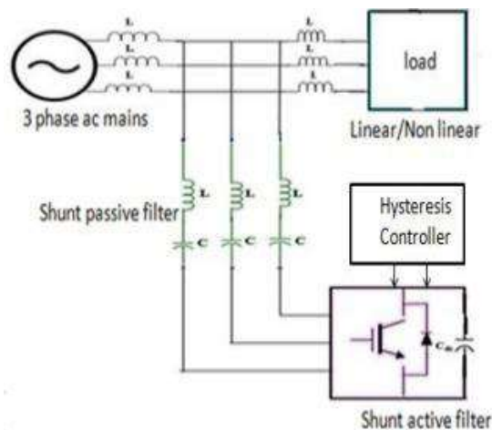
Figure 10: Hybrid filter connected to grid
