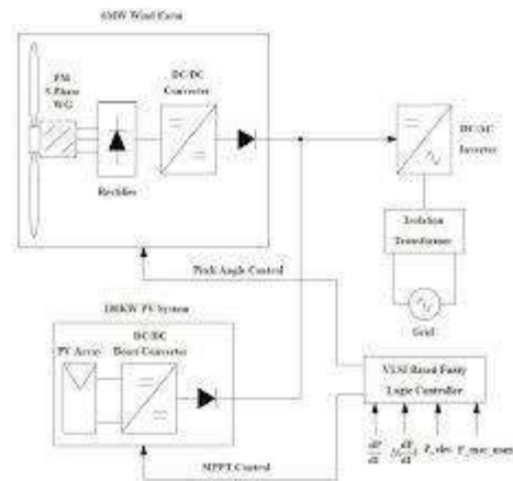
Figure 3: Block diagram of Hybrid system with Fuzzy logic controller
