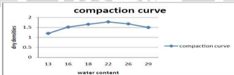
Fig: 3.1 Compaction curve
