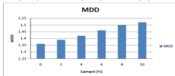
Fig : 3.14 Variation of MDD with % of cement
