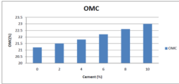
Fig: 3.9 Variation of OMC with % of cement.
