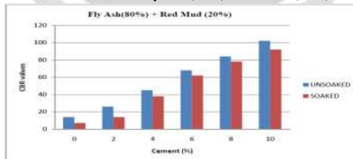
Fig : 3.24 variation of CBR values with various percentage of cement
