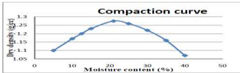
Fig: - 3.4 Compaction curve of NTPC Fly Ash
