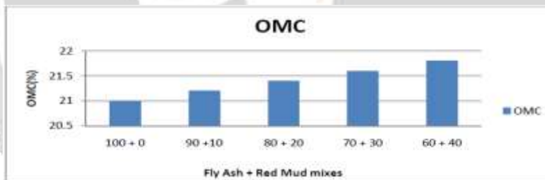
Fig : 3.5 OMC Curve With Different Combinations Of Red Mud + Fly Ash
