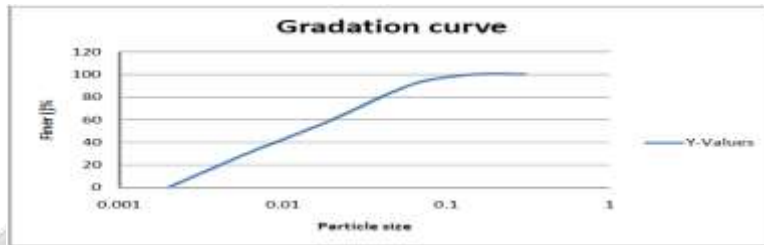
Fig : 3.2 Gradation curve for Red Mud
