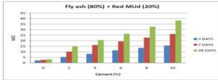
Fig: 3.18 Variations of UCC with different percentage of cement
