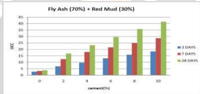
Fig: 4.19 Variations of UCC with different percentage of cement
