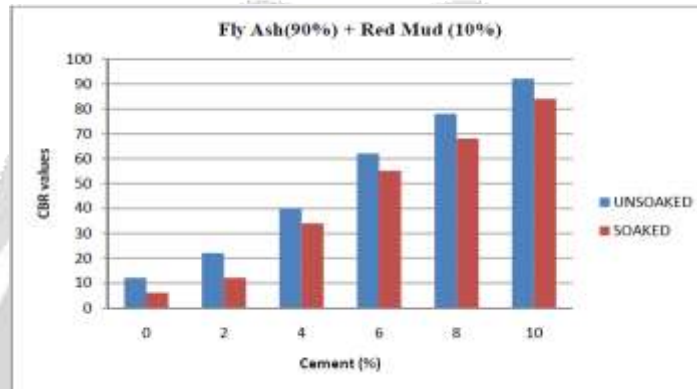
Fig : 3.21variation of CBR values with various percentage of cement
