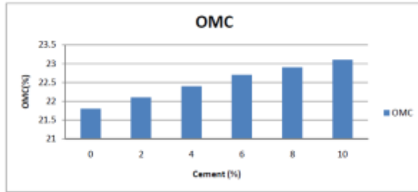
Fig : 3.15 Variation of OMC with % of cement
