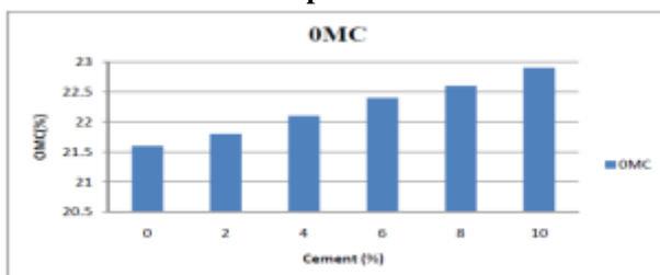
Fig : 3.13 Variation of OMC with % of cement
