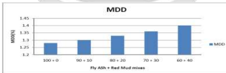
Fig: 3.6 MDD Curve with Different Combinations Of Red Mud + Fly Ash
