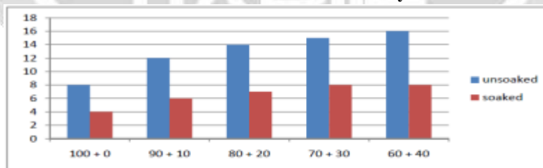
Fig: 3.8 variation of CBR values with various percentage of Fly Ash – Red Mud
