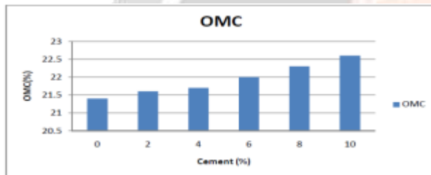
Fig: 3.11 Variation of OMC with % of cement
