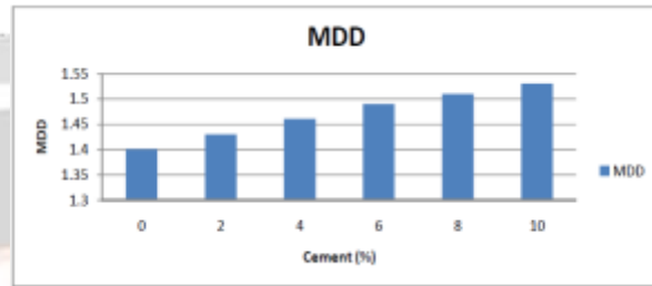
Fig : 3.16 Variation of MDD with % of cement
