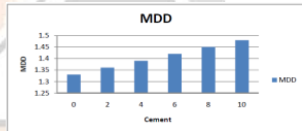
Fig:3.12 Variation of MDD with % of cement
