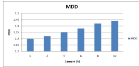
Fig: 3.10 Variation of MDD with % of cement
