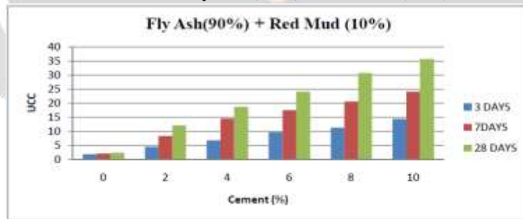
Fig: 3.17 Variations of UCC with different percentage of cement
