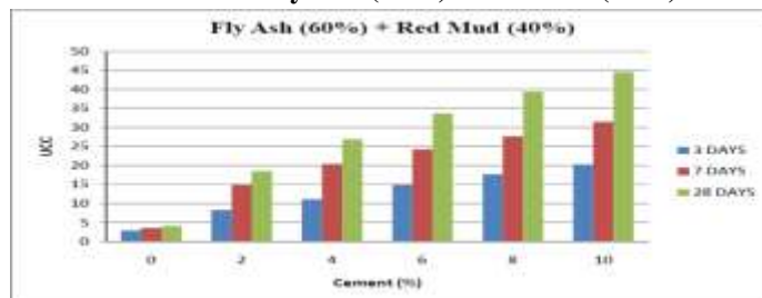
Fig: 3.20 Variations of UCC with different percentage of cement
