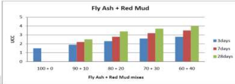
Fig: 3.7 UCC Curve with Different Combinations Of Fly Ash + Red Mud
