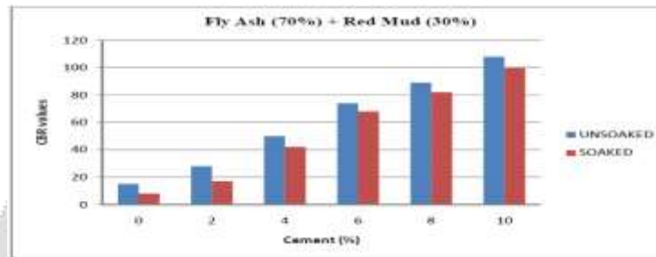
Fig:3.23 variation of CBR values with various percentage of cement
