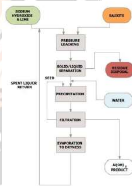
Fig.1(a) BAYER'S PROCESS
