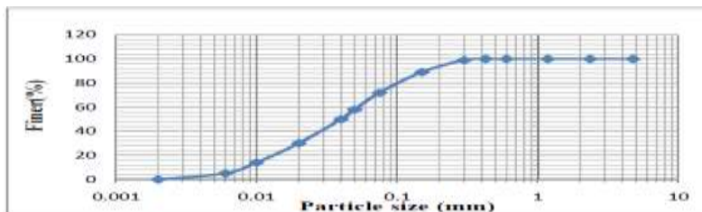
Fig:- 3.3 Gradation Curve of NTPC Fly Ash
