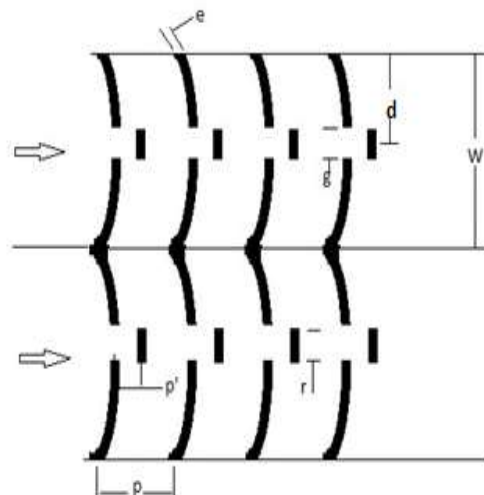
Fig. 2 Schematic diagram of (a) Continuous Ribs and (b) Broken double arc rib with stagger Piece
