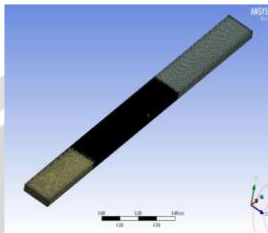
Fig.3 Meshing of computational Domain for arc-rib with gap
