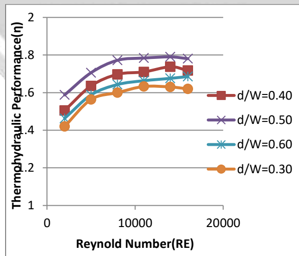
Fig.5 Thermo-hydraulic performance parameter as a function of Reynolds Number for different relative gap position (d/W)
