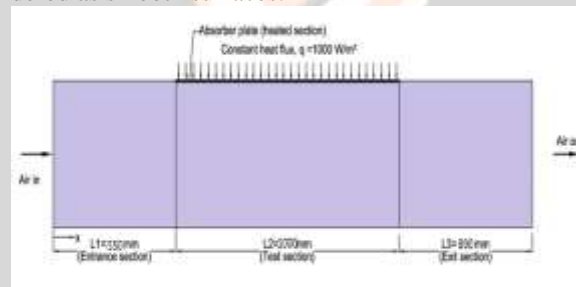
Fig.1. Showing the geometric dimension of the working model
