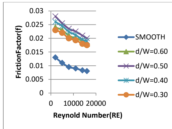
Fig. 6 Comparison between Friction factor and Reynolds number at different gap position (d/W)
