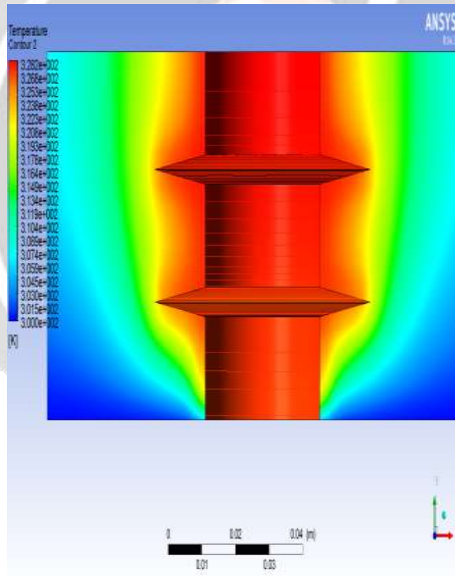
Fig.6.Contours of Total Temperature For Tube With Rectangular Fin
