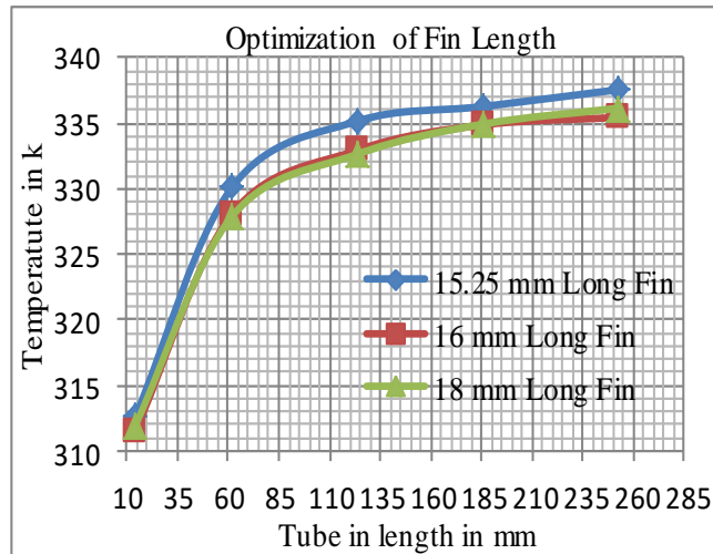
Graph No.1..Optimization of Fin Length
