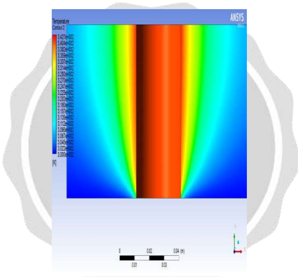
Fig.5. Contours of Total Temperature For Tube Without Fins
