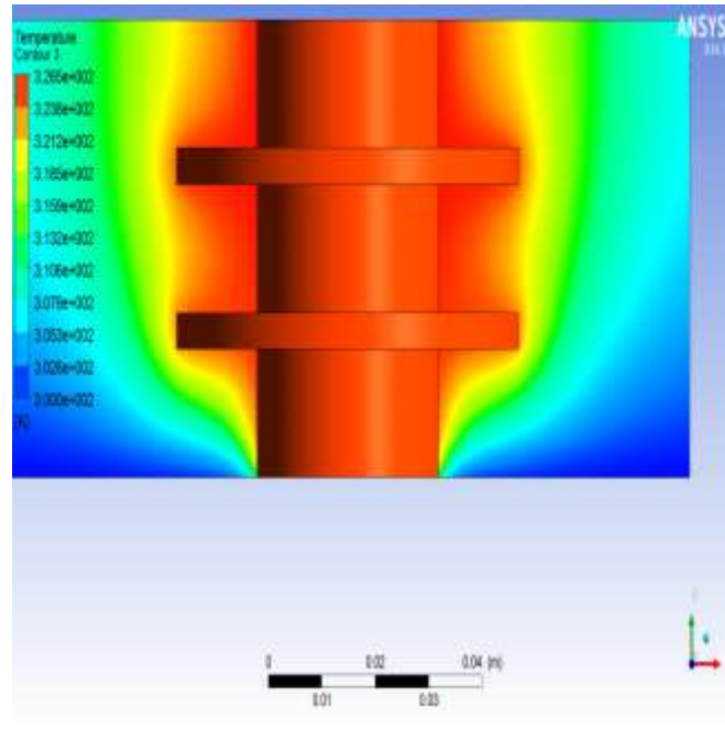
Fig.6.Contours of Total Temperature For Tube With Rectangular Fin
