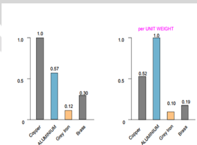
Fig 2.1 thermal conductivity of Al compared with other metal
