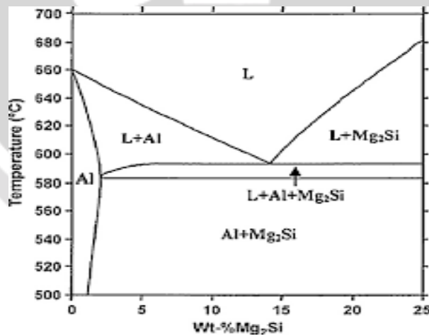
Fig 3.1(c) phase diagram for Al-Mg 2 Si
