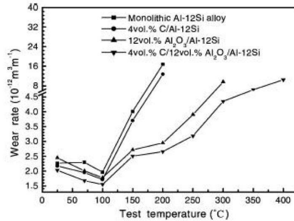
Fig 2.1(b) wear rate
