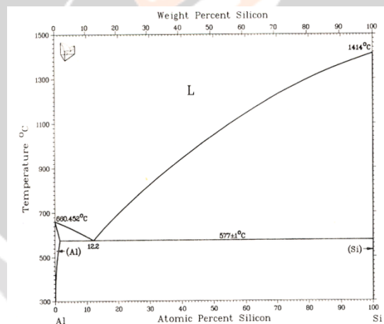
Fig 3.1(a) phase diagram for Al-Si
