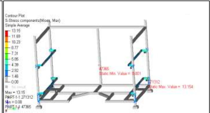
Fig 08 – Case 1_Stress plot without stacking
