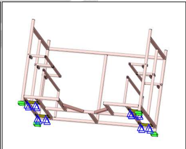
Fig 4 – Boundary condition
