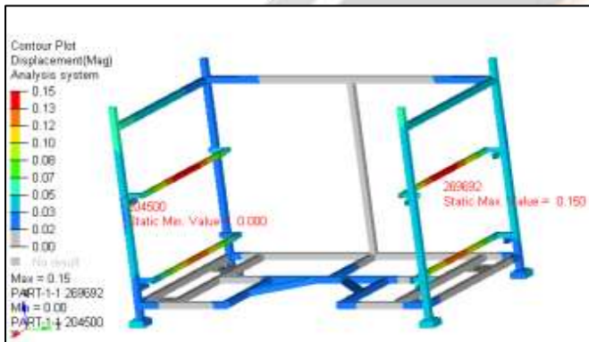
Fig 09 – Case 1_Displacement plot with stacking
