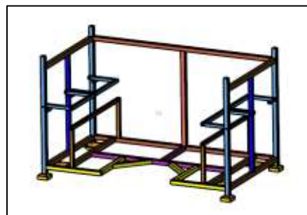
Fig 1 – Existing trolley design
