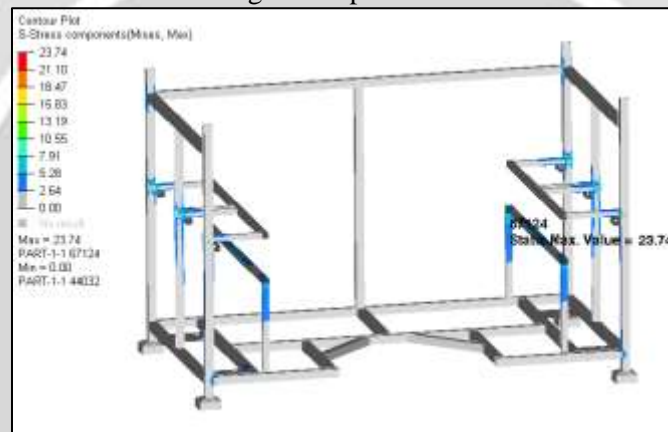
Fig 6 - Stress distribution (Von-mises)
