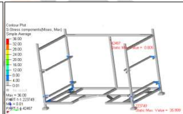
Fig 10 – Case 1_Stress plot with stacking
