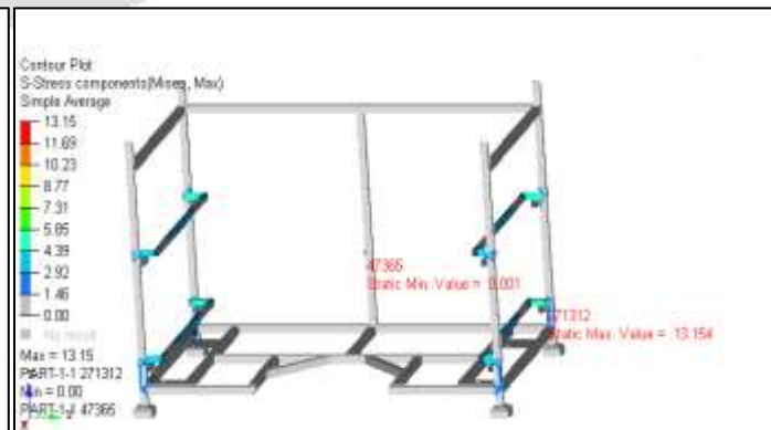
Fig 26 – Case 4_Stress plot without stacking
