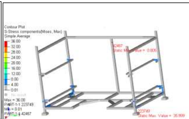
Fig 28 – Case 4_Stress plot with stacking
