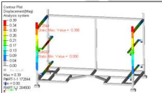
Fig 20 – Case 3_Displacement plot without stacking
