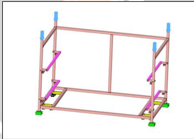
Fig 24 – Case 4_Load and boundary condition
