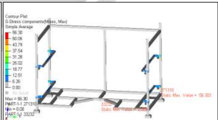
Fig 21 – Case 3_Stress plot without stacking
