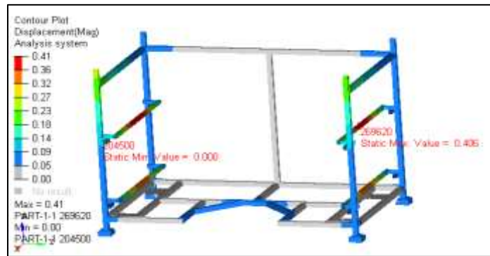
Fig 22 – Case 3_Displacement plot with stacking
