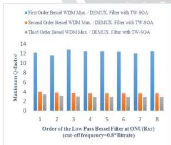
Fig-3:- Comparative analysis for various order of Bessel filter
