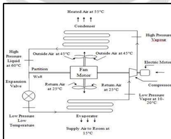
Fig -1: Schematic diagram of Winter Air Conditioner
