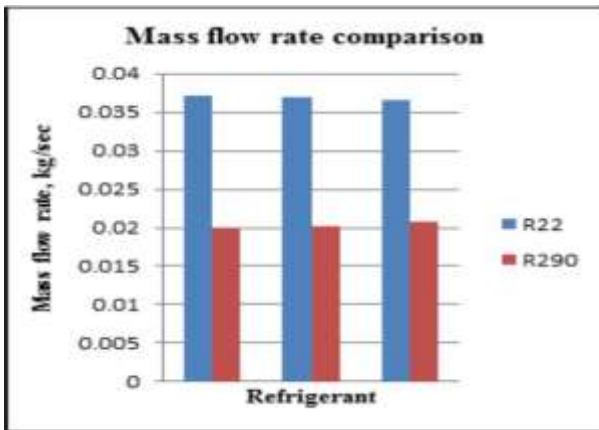
Chart -1: Mass flow rate comparison
