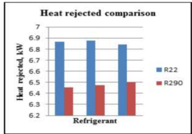
Chart -4: Heat rejected comparison
