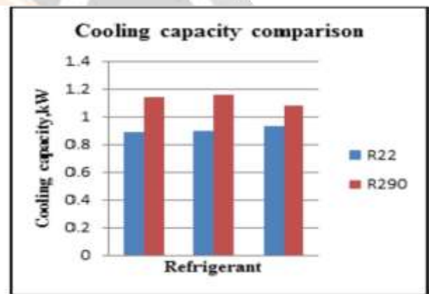
Chart -5: Cooling capacity comparison
