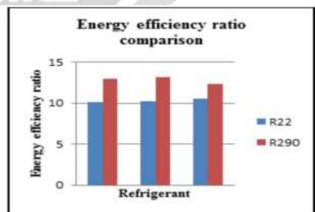
Chart -6: Energy efficiency ratio comparison
