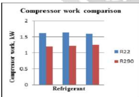
Chart -3: Compressor work comparison
