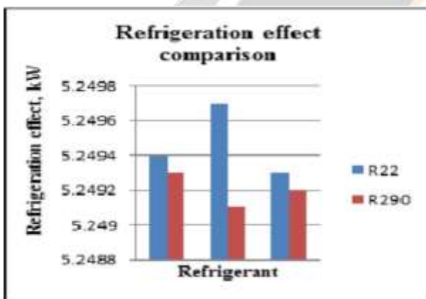
Chart -2: Refrigeration effect comparison
