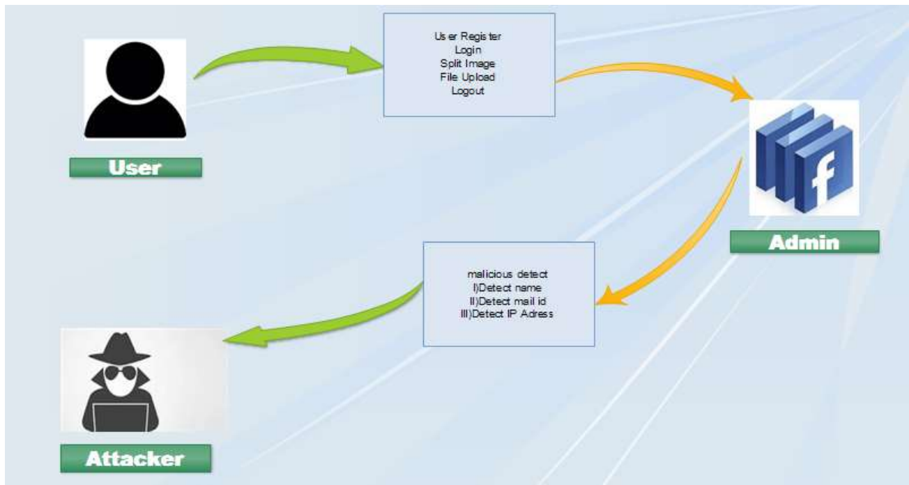
Fig 1. Architecture.
