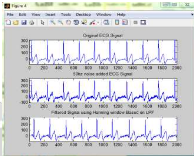
Fig-5-Filter signal using Hanning Window
