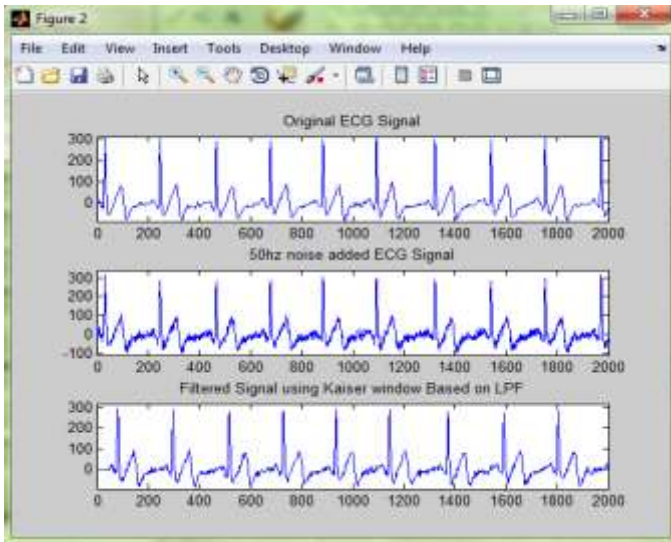
Fig. 4. – Filter signal using Kaiser Window
