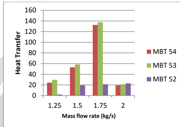
Fig 3 Graph of mass of flow rate VS heat transfer
