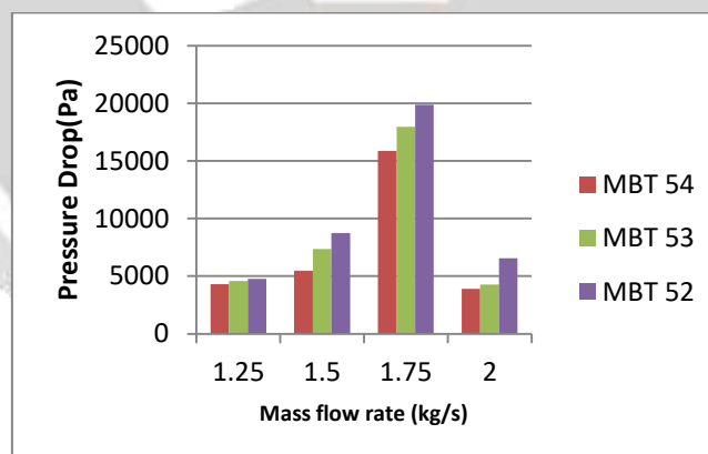
Fig. 4 Graph of Pressure drop VS mass flow rates
