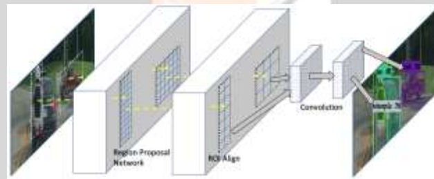
Figure 3: Architecture of Mask R-CNN.
