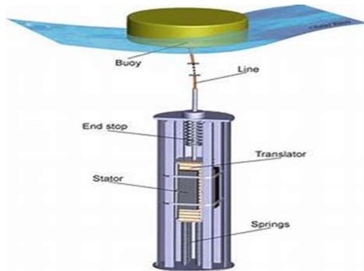
Fig 2: Schematic Diagram of Buoy.
