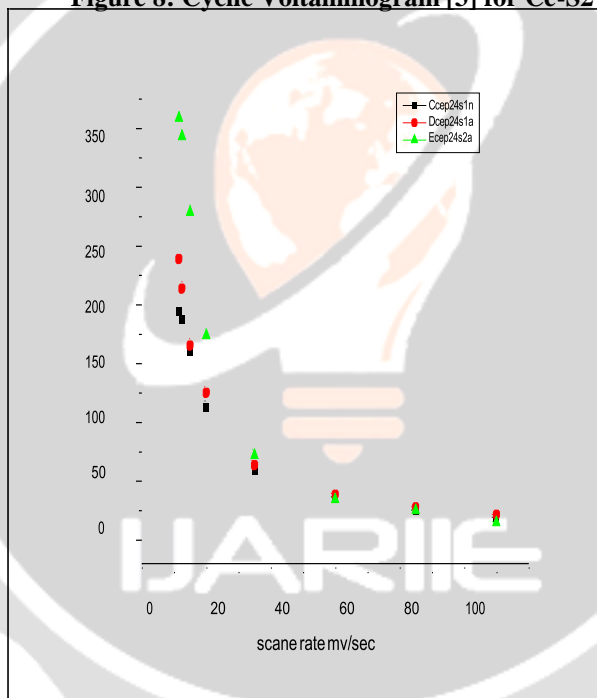
Figure 8: Cyclic Voltammogram [3] for Ce-S2
