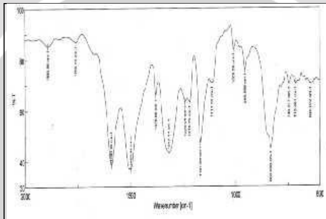
Figure 3: FTIR of Ce doped PANI in Range 600 to 2000 \text{cm}^{-1}
