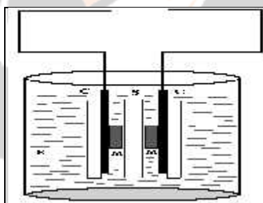
Figure 5: Schematic Diagram of Double Layer Capacitor Cell
