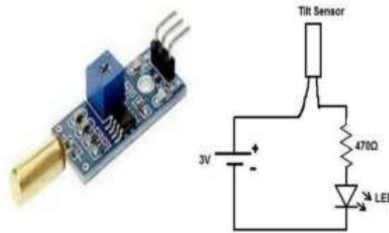
Fig 5. Tilt Sensor [SW – 520D]
