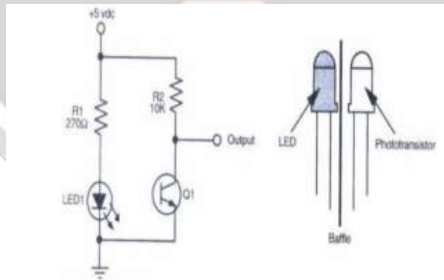
Fig 6.IR Sensor- REES52
