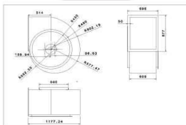
Fig (08) Drafting of Blower Casing
