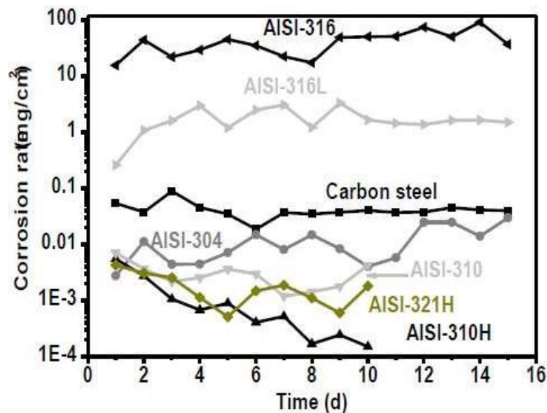
Fig (04): Comparison of the corrosion rate of some stainless steel materials and carbon steel exposed to LiBr-H 2 O (50% wt) at 80°C. Table1. Nominal composition of some studied materials under Li-Br conditions (wt. %).
