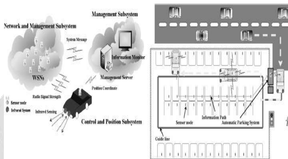
Figure 3. Architecture and the operation procedure of the automatic vehicle parking system.
