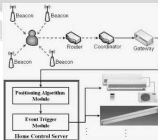
Figure 5. System Architecture
