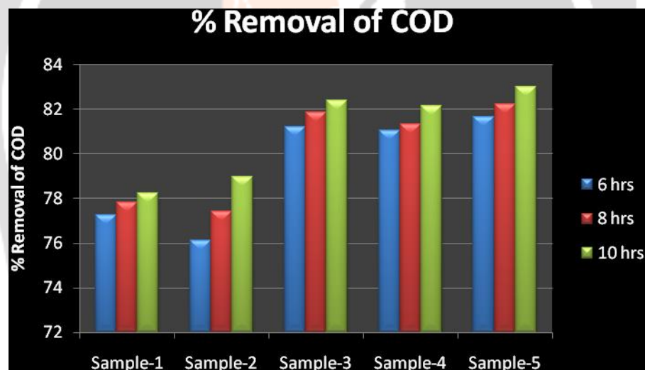
Figure 8: % Removal of COD
