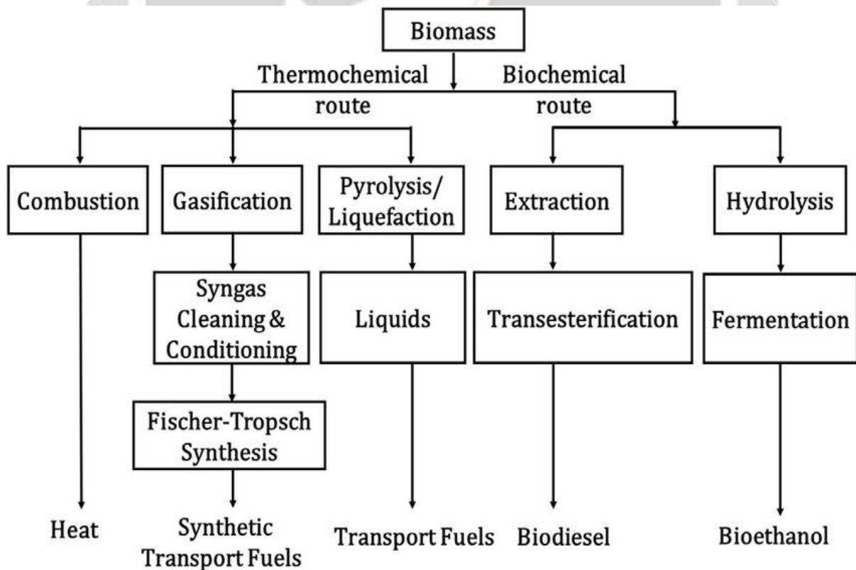
Fig. 3 Thermochemical and biochemical pathways [6]
