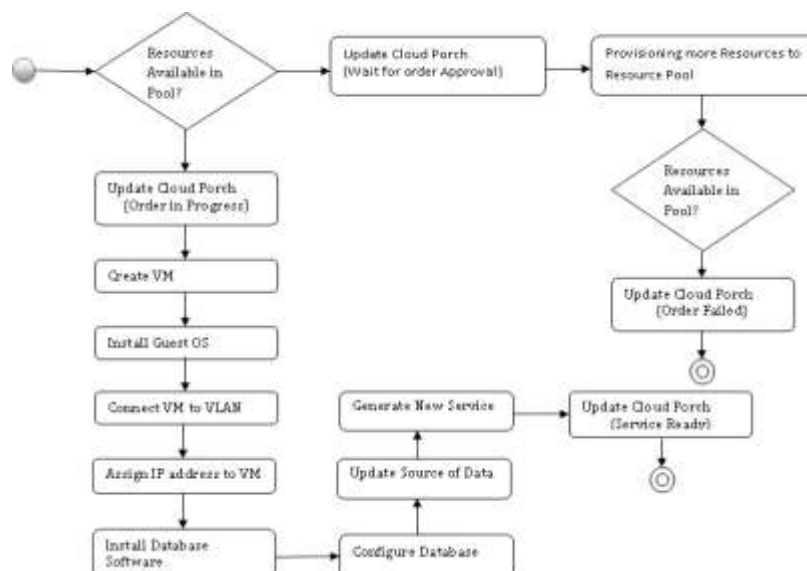
Figure 4.1: Algorithm Steps - Service Coherence
