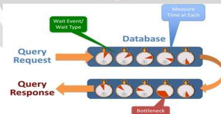
Figure 5.1: Response Time for Query Process Analysis
