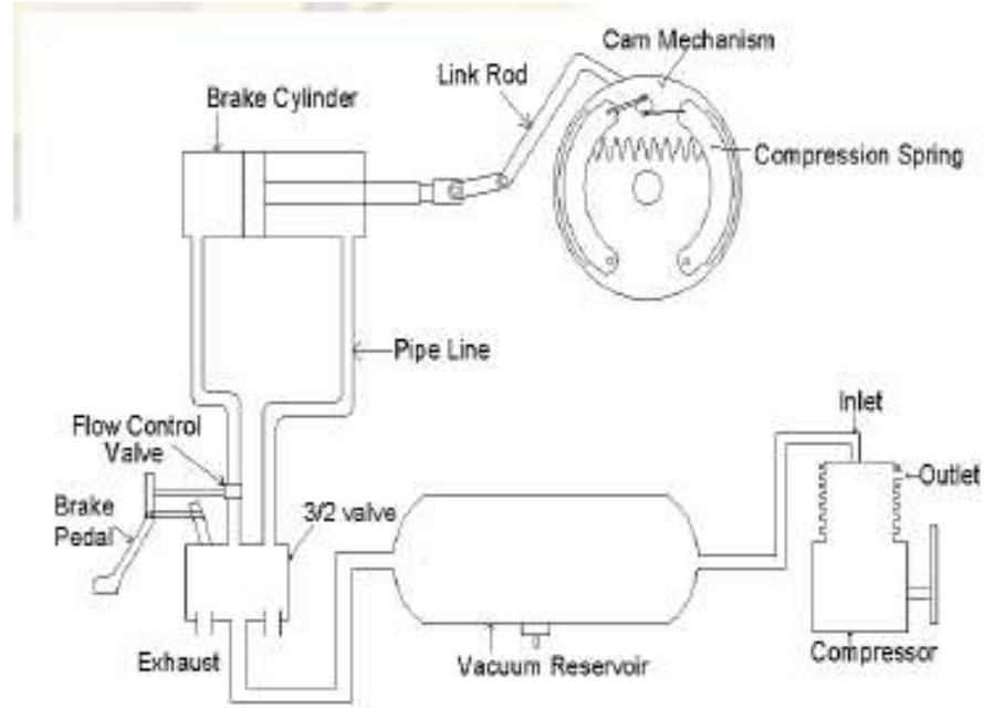
Vacuum braking system
