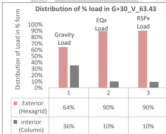
Figure 11. Distribution of % load in G+30_V_63.43°
