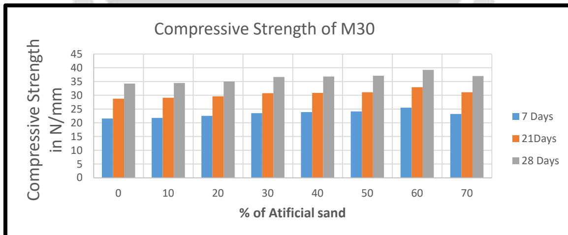
Variation of compressive strength after 7,14 and 28 days curing for M30
